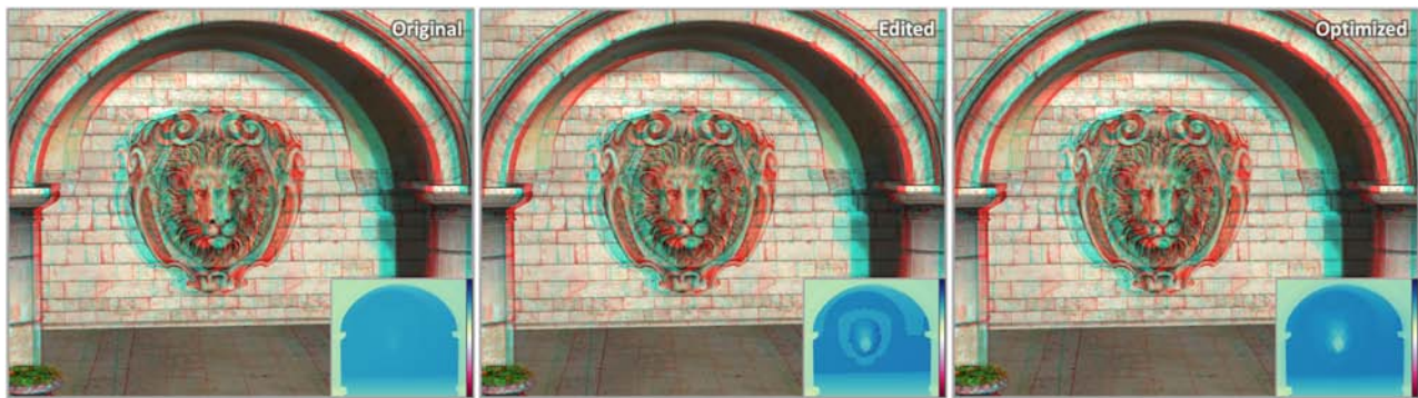
Figure 1: Left: Original stereographic image with disparity map inset Middle: An edited version, where we increased the roundness of the lion head and moved the background wall away from the viewer, presents depth-cue conflicts where the edited elements meet. Right: Our optimization procedure preserves edits while removing inconsistencies. 🇧🇪 🇩🇪
