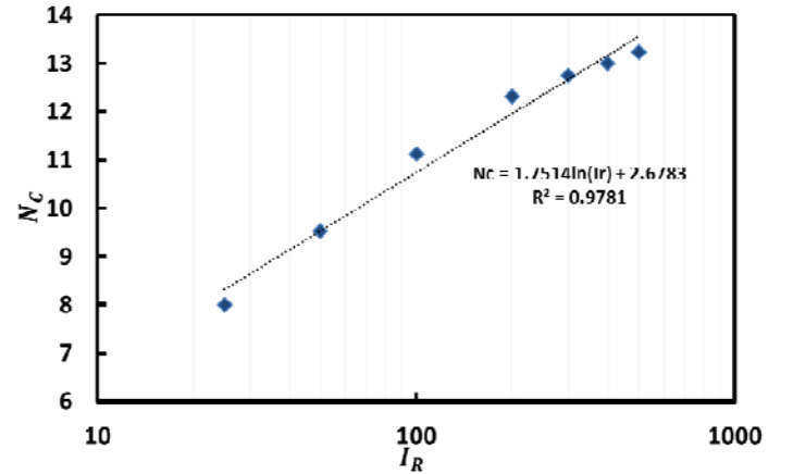
Figure 5. Variation of cone factor with rigidity index
