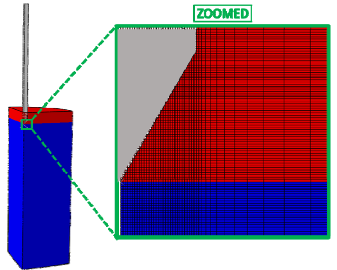
Figure 2. Finite element model of cone penetration analysis
