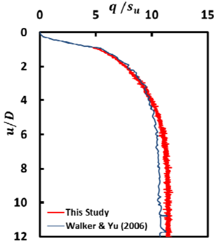
Figure 3. Comparison of penetration resistance in single-layer clay from this study and Walker and Yu (2006)
