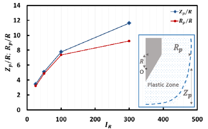
Figure 8. Variation of plastic zone extent with rigidity index of the soil
