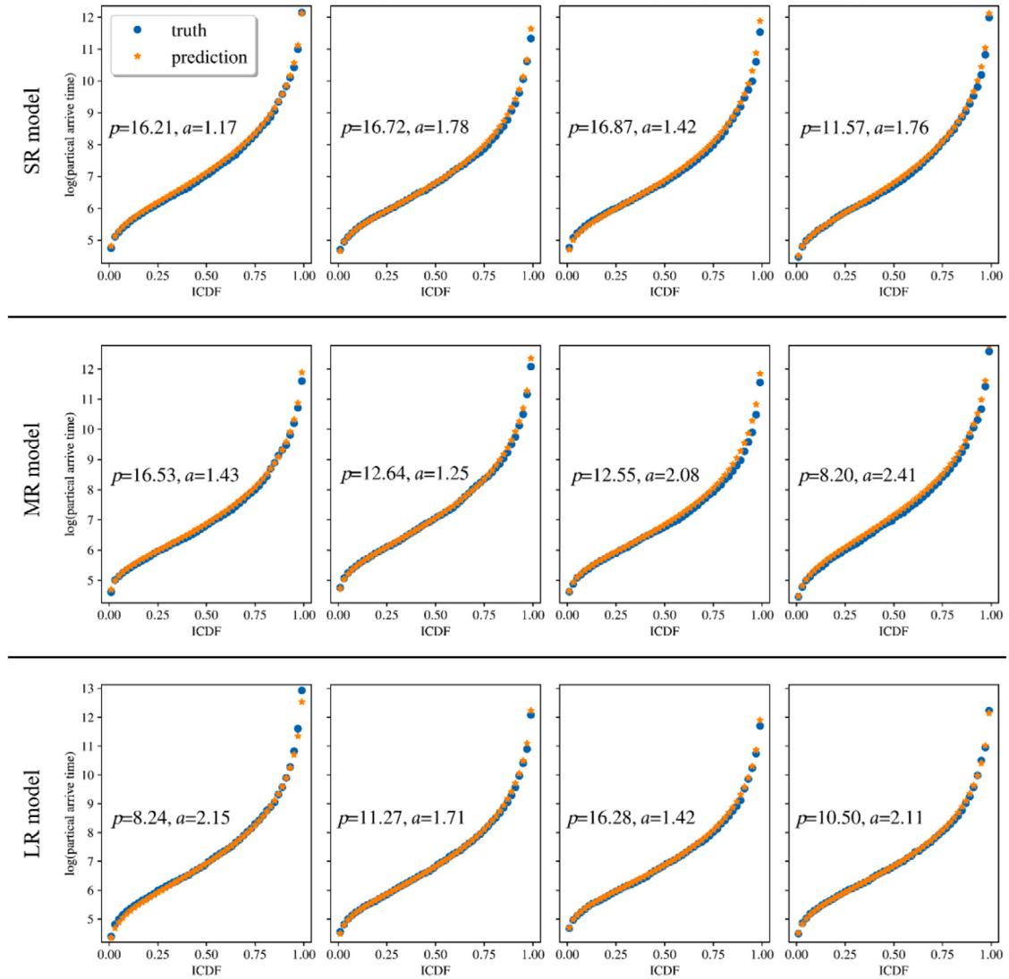
Fig. 6. Examples of iCDFs computed with the reference PBPT solver (denoted as truth) and the SR (top), MR (middle), and LR (bottom) regionalized surrogate models (denoted as prediction) for several realizations of parameters a and p drawn from the definition domains of the respective models.
