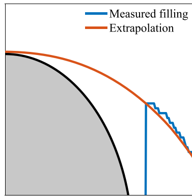
Fig. 24. Example of the extrapolation used at the upstream cavity edge for case C3 in Fig. 23a.
