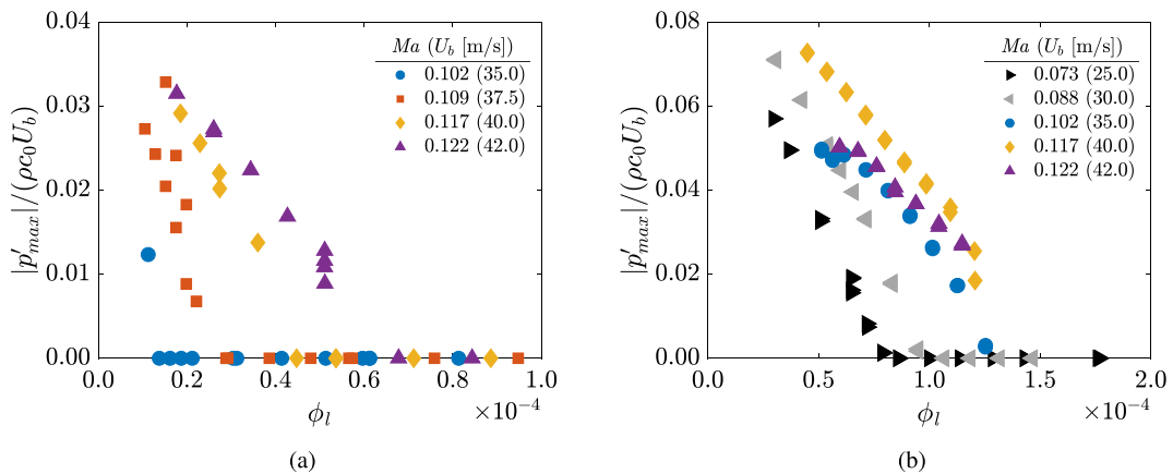
Fig. 7. Dimensionless acoustic whistling amplitude as a function of the liquid volume fraction \phi_l for pipes with a reference corrugation geometry A (a) and the enlarged geometry D (b, see Fig. 3).
