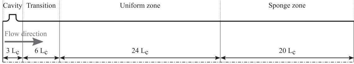
Fig. 14. Numerical domain used for simulations of the cavity with geometry A. The cavity zone is densely meshed, followed by a transition to a uniform grid size. The sponge zone is applied to reduce reflections from the outlet.
