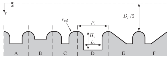
Fig. 3. Schematic representation of the different cavity geometries used in the present study. The cavity size in the figure is exaggerated with respect to the pipe diameter. Definition of the cavity sizes is given in geometry D, values are found in Table 1 .
