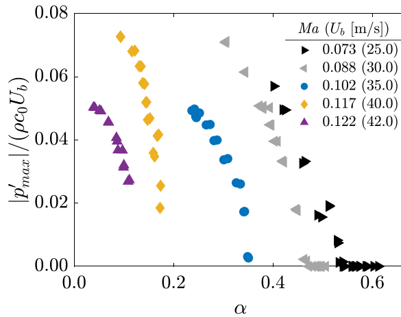
Fig. 11. Dimensionless whistling amplitude as a function of the liquid filling fraction \alpha , for geometry D, with water injection.
