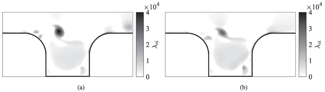
Fig. 20. Vortices traveling over the cavity mouth, visualized using the swirling strength criterion [54]. The amplitude of the perturbation velocity is |u'_{ac}|/U_b = 0.1 (a) and 0.025 (b), for a bulk velocity of 40 m/s.
