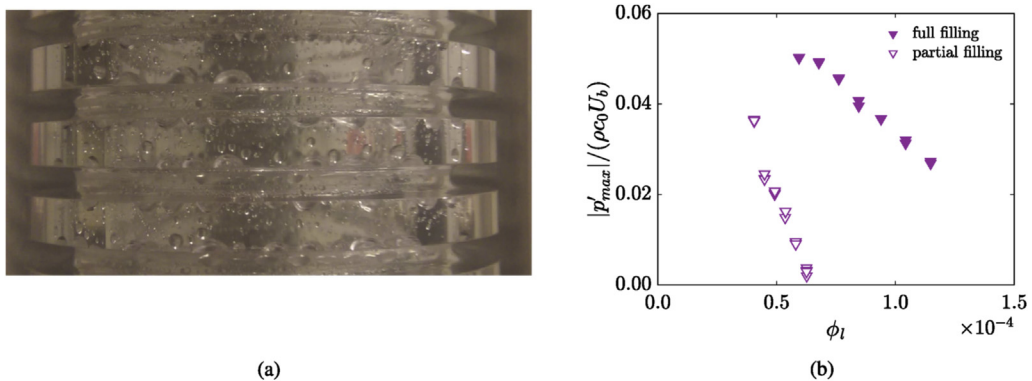
Fig. 13. (a) Qualitative view of the filling pattern for a corrugated pipe with geometry D after hydrophobic wall treatment. (b) Dimensionless whistling amplitude as a function of the liquid volume fraction, for two-phase water-air flow through a pipe with corrugation geometry D. When the axisymmetry of the filling is broken due to a non water-wetting coating of the wall (open markers), the required liquid volume fraction to make whistling disappear is substantially reduced.
