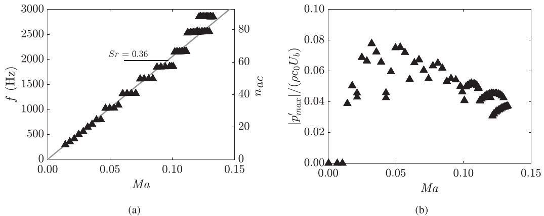
Fig. 5. (a) Whistling frequency ( f ) as a function of the Mach number for geometry A, showing the step-wise increase in whistling frequency. The solid line represents Sr = 0.36 . The right hand side y-axis shows the acoustic resonance mode n_{ac} of the pipe system (see Eq. (2)), associated to the whistling frequency. (b) Dimensionless amplitude of the acoustic standing wave ( |p'_{max}| / (\rho c_0 U_b) ) as a function of the Mach number for geometry A.
