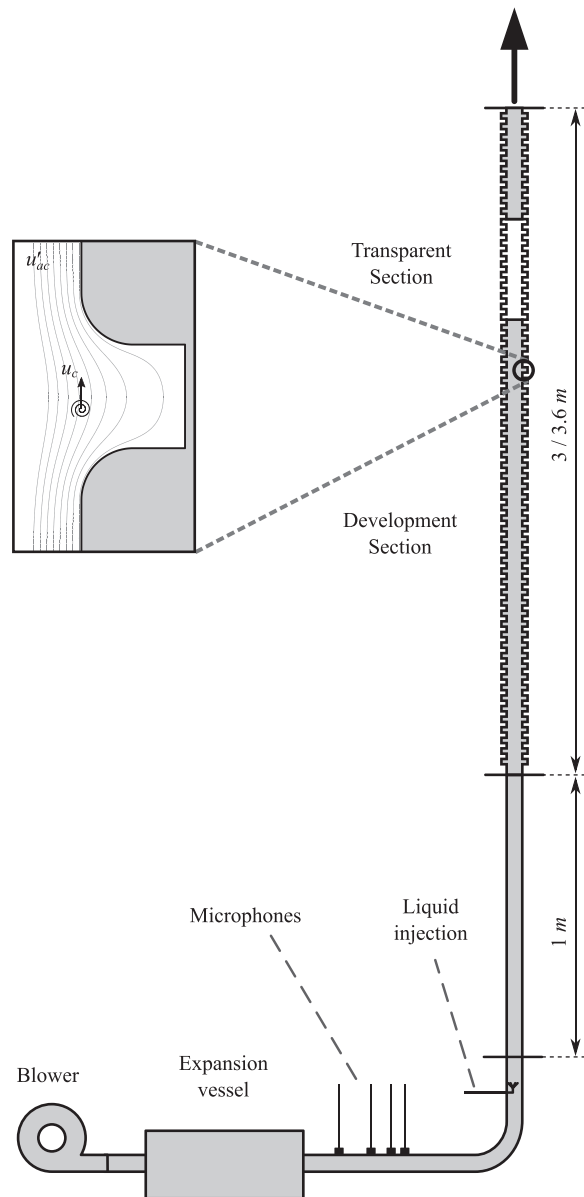
Fig. 2. Schematic representation of the experimental set-up. The gas flow is created by a blower, followed by an expansion vessel to prevent the blower noise to reach the test section and to provide a large reflection coefficient boundary condition at the pipe inlet. The flow subsequently enters the acoustic measurement section. Liquid is injected with a spray nozzle at the pipe centerline. The corrugated section is vertical and flow is in upward direction. The corrugated section is partly transparent for the optical measurements. The insert shows a schematic representation of the acoustic streamlines over a cavity structure, with a coherent vortex traveling in the cavity mouth with velocity u_c .
