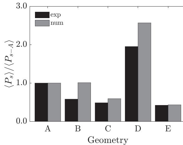
Fig. 21. Normalized acoustic source power obtained from URANS simulations and experiments, for the different geometries listed in Fig. 3 and Table 1.
