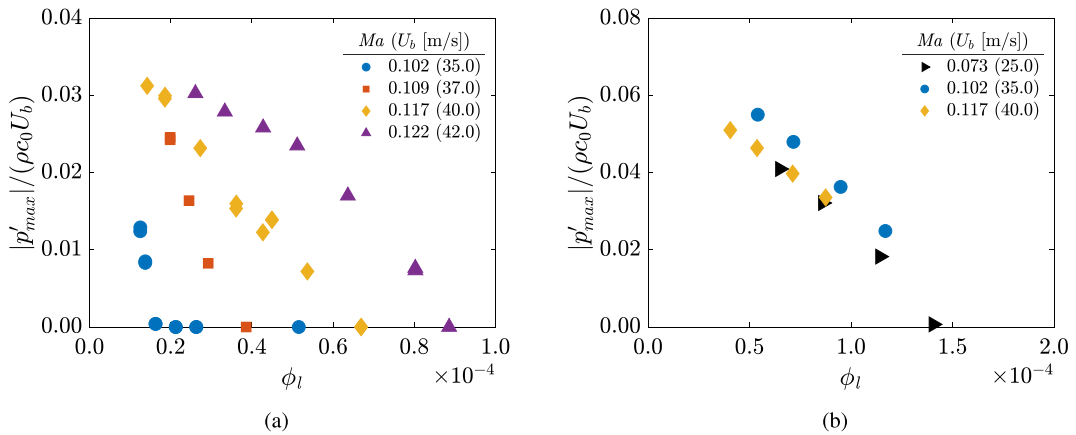
Fig. 9. Dimensionless acoustic whistling amplitude as a function of the liquid volume fraction \phi_l for corrugated pipes with geometry A (a) and D (b). Mono-ethylene glycol (MEG) is used in these measurements, instead of water (compare to Fig. 7).
