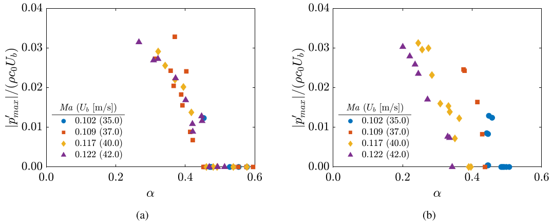
Fig. 10. Dimensionless whistling amplitude as a function of the liquid filling fraction \alpha , for geometry A with water (a) and MEG (b) injection.
