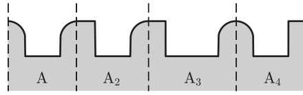
Fig. 22. Geometries based on geometry A, used to assess the effect of edge rounding on acoustic the source power.
