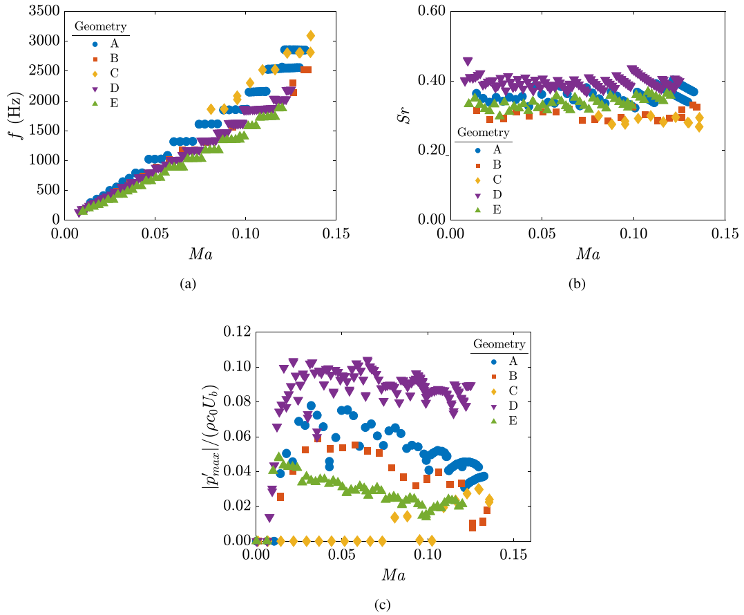
Fig. 6. Whistling frequency, whistling Strouhal number and amplitude as a function of the Mach number, for the geometries depicted in Fig. 3. (b) Whistling Strouhal number as a function of the Mach number, for the geometries depicted in Fig. 3. (c) Dimensionless acoustic amplitude as a function of the Mach number, for the geometries depicted in Fig. 3.
