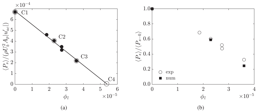
Fig. 23. (a) Acoustic source strength obtained from experiments with corrugation geometry A, versus the liquid volume fraction \phi_l . The bulk gas flow velocity U_b is 40 m/s. Experimentally obtained filling profiles for four values of the liquid volume fraction are used to numerically obtain the source strength (C1–4). (b) Comparison of the normalized source power obtained from experiments and single phase simulations, as a function of liquid volume fraction for geometry A at a gas flow velocity of 40 m/s.
