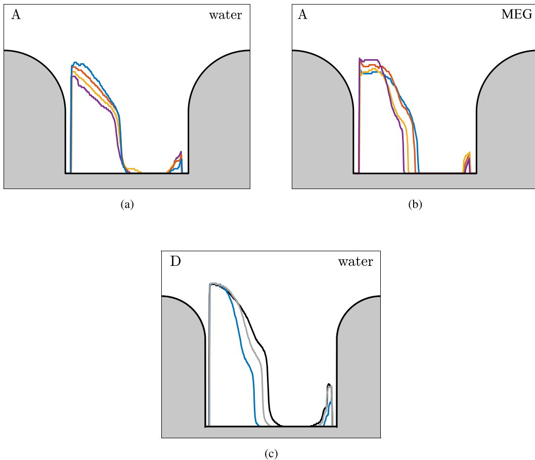
Fig. 12. Averaged liquid filling profiles for geometry A with water injection (a) and MEG injection (b) and for geometry D with water injection (c). The profiles are for liquid flow rates where whistling has just disappeared. The colors correspond to the colors used in Fig. 10a, b, and 11, respectively. (For interpretation of the references to color in this figure legend, the reader is referred to the Web version of this article.)
