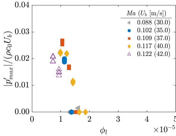
Fig. 8. Dimensionless acoustic whistling amplitude as a function of the liquid volume fraction \phi_l for corrugated pipes with geometry C (open markers) and E (closed markers).
