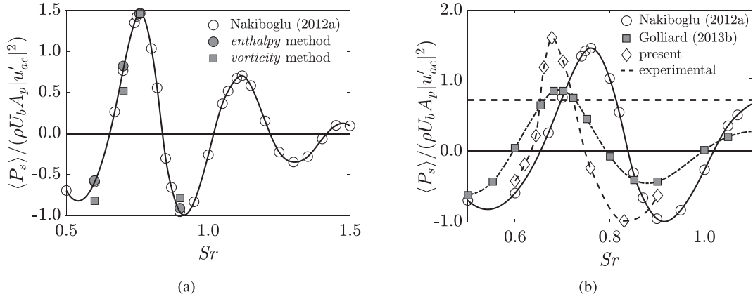
Fig. 15. (a) Comparison of the dimensionless acoustic source power as a function of the whistling Strouhal number obtained with the enthalpy and vorticity method, compared to results from literature [12,51] at a Reynolds number of 4 \times 10^3 (a) and 4 \times 10^4 (b). The experimentally obtained source power, depicted in (b), is also taken from Nakiboglu et al. [12].
