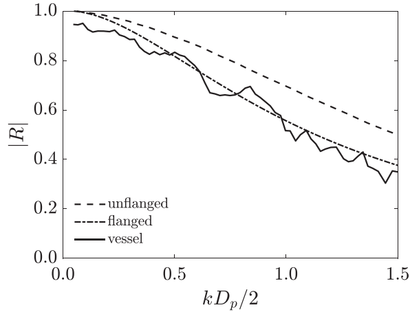
Fig. 1. Experimentally obtained reflection coefficient for the expansion vessel, compared to the reflection coefficient from an unflanged [31] and flanged pipe [32].
