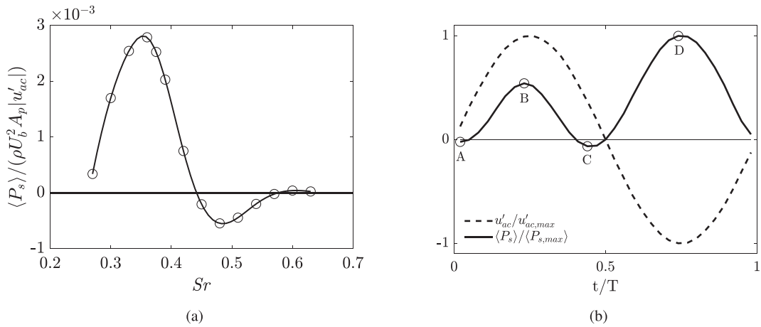
Fig. 16. (a) Dimensionless acoustic source power as a function of whistling Strouhal number for geometry A, at a perturbation amplitude of |u'_{ac}|/U_b = 0.1 , and a bulk velocity of 40 m/s. (b) Temporal distribution of the source strength (—) and the acoustic perturbation amplitude (---) over a full period of the perturbation cycle at the peak-whistling Strouhal number. The bulk gas velocity is 40 m/s, the perturbation amplitude amounts 10% of the bulk velocity. Values are normalized with the maximum values obtained in a whistling period. The points A, B, C and D relate to Fig. 17.
