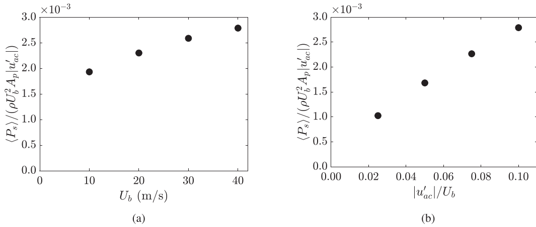
Fig. 19. Dimensionless acoustic source power as a function of the gas flow velocity (a) and the perturbation amplitude (b).
