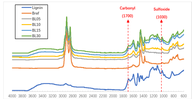
Fig. 2. IR spectra of lignin-modified bitumen.
