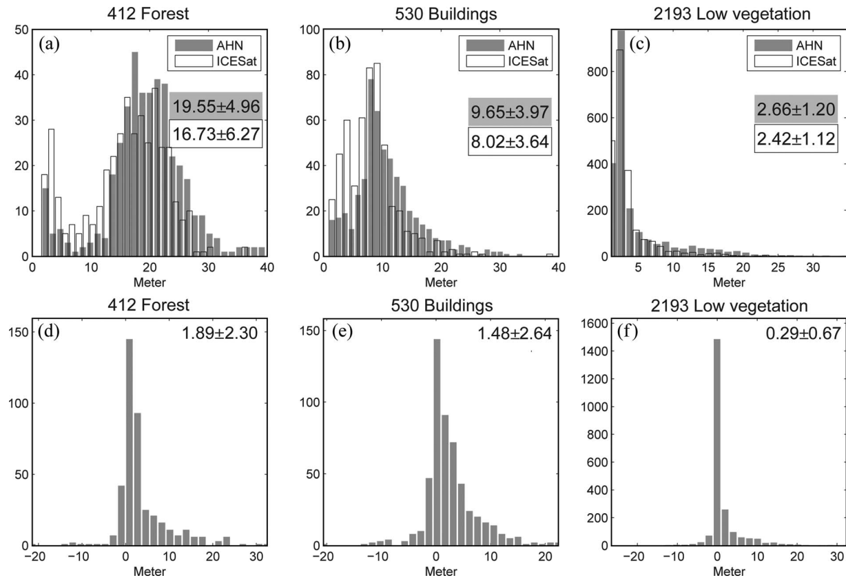
Fig. 12. Histograms of feature heights extracted from AHN and ICESat data for (a) forest, (b) buildings, and (c) low vegetation. (Gray) Histograms of the AHN feature heights. The ICESat histograms are bounded by a solid black line. For both AHN and ICESat, the mean value and standard deviation are given in the corresponding text boxes. Moreover, the histograms of H_{LM-WB} feature height differences between AHN and ICESat data are shown in (d)–(f) for different terrain classes. In each plot, the Median/MAD value is indicated.
