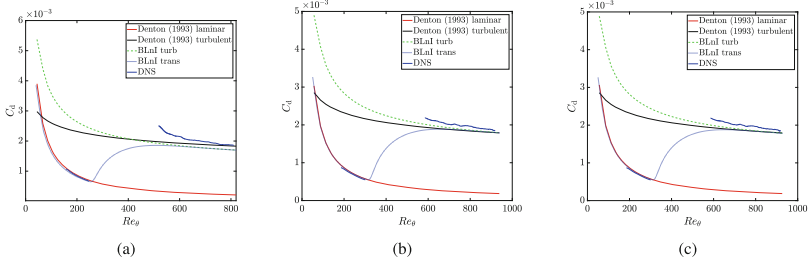
Fig. 2. Dissipation coefficient C_d vs Re_\theta for the cases (a) air , (b) iMM and (c) niMM . Results from turbulent and transitional simulations conducted with BLnI as well as those obtained from the DNS are plotted. Correlations by Denton and Schlichting are also displayed.
