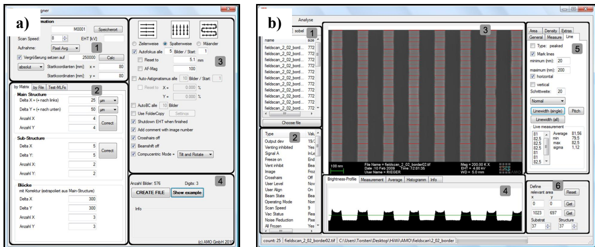
Figure 1. In-house solutions for a) automated SEM image acquisition and b) analysis at AMO by the SEMacroDesigner and SEMalyser tools. [1]
