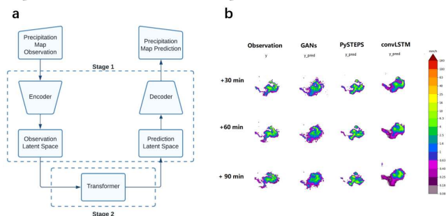
Fig. 1. (a) Proposed model structure. (b) Example prediction of precipitation intensity for 30, 60 and 90 min using nowcasting methods GAN, PySTEPS and convLSTM [1], [5], [6].
