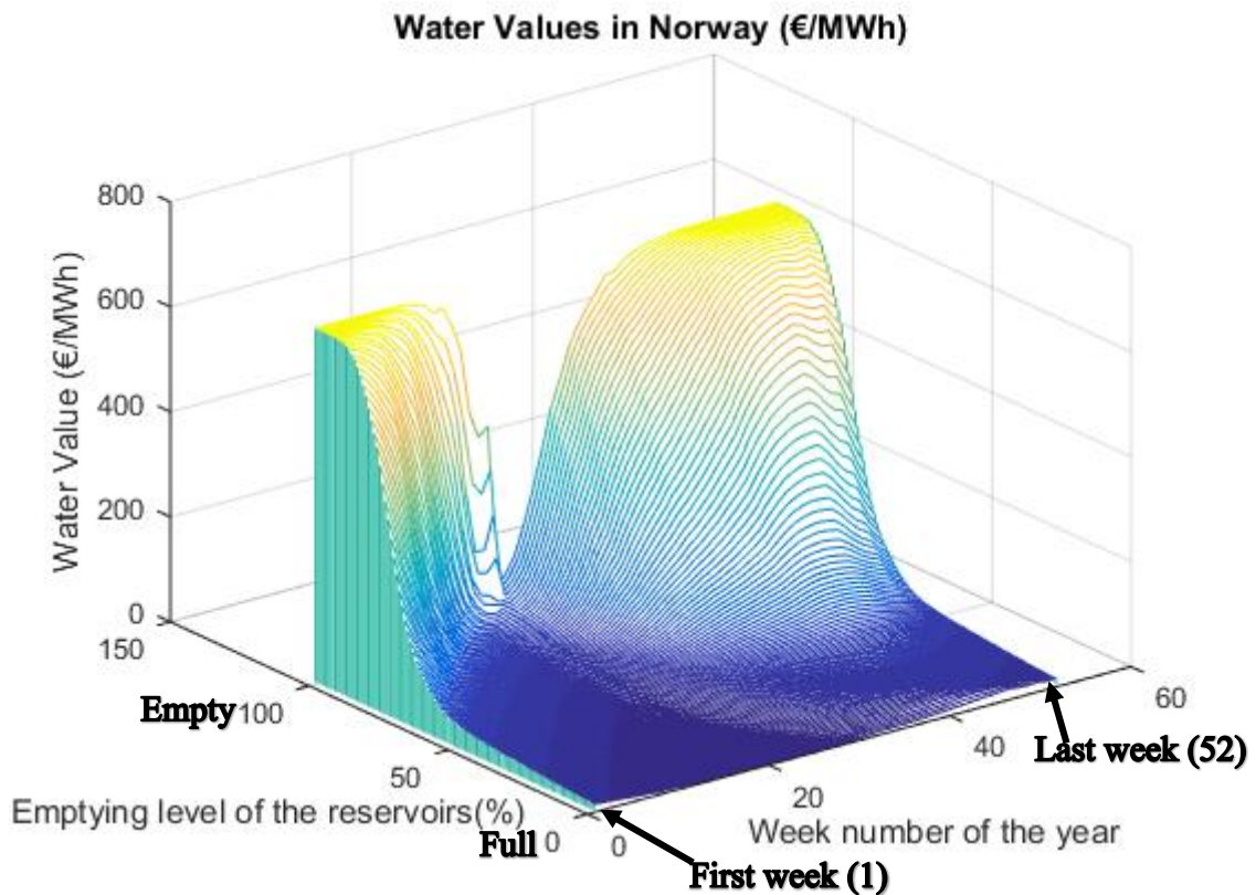
Figure 18. Water values in Norway.
