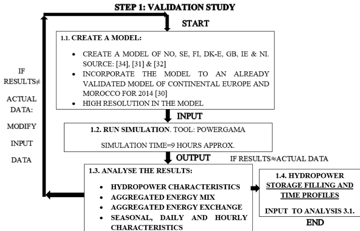
Figure 1. Flow chart of the first step of this Master Thesis.
