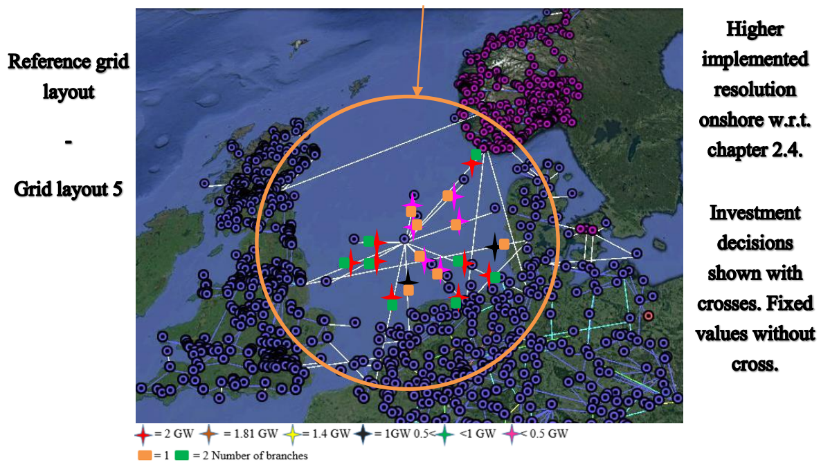
Figure 50: Created reference grid layout.
