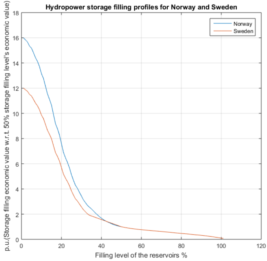
Figure 19. Storage filling profiles for Norway and Sweden.
