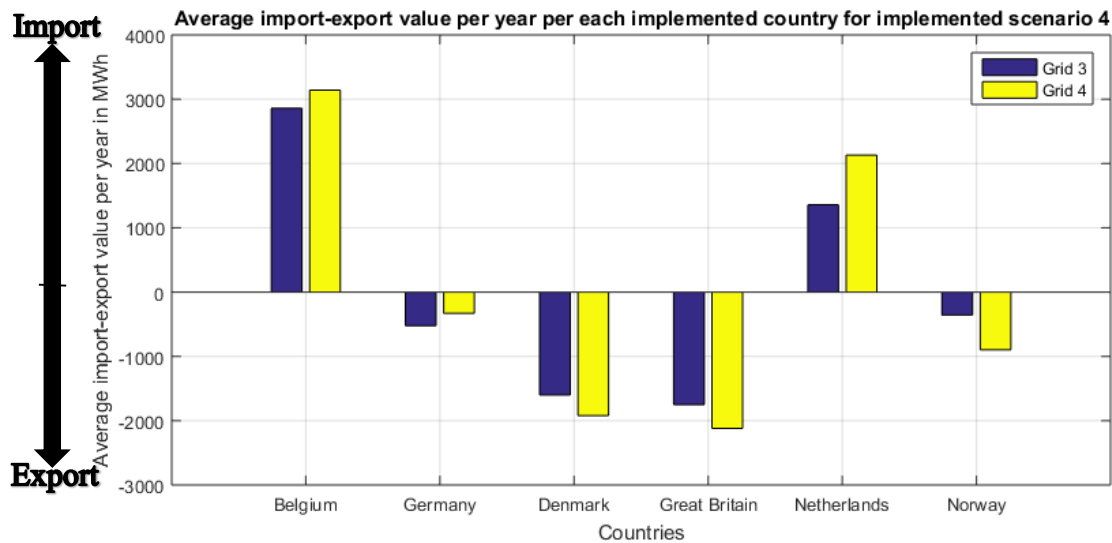
Figure 55. Average import-export value per country (Sn 4)
