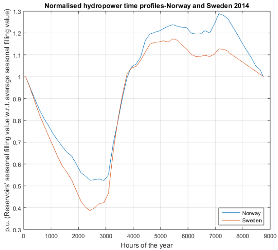
Figure 20. Storage time profiles for Norway and Sweden.
