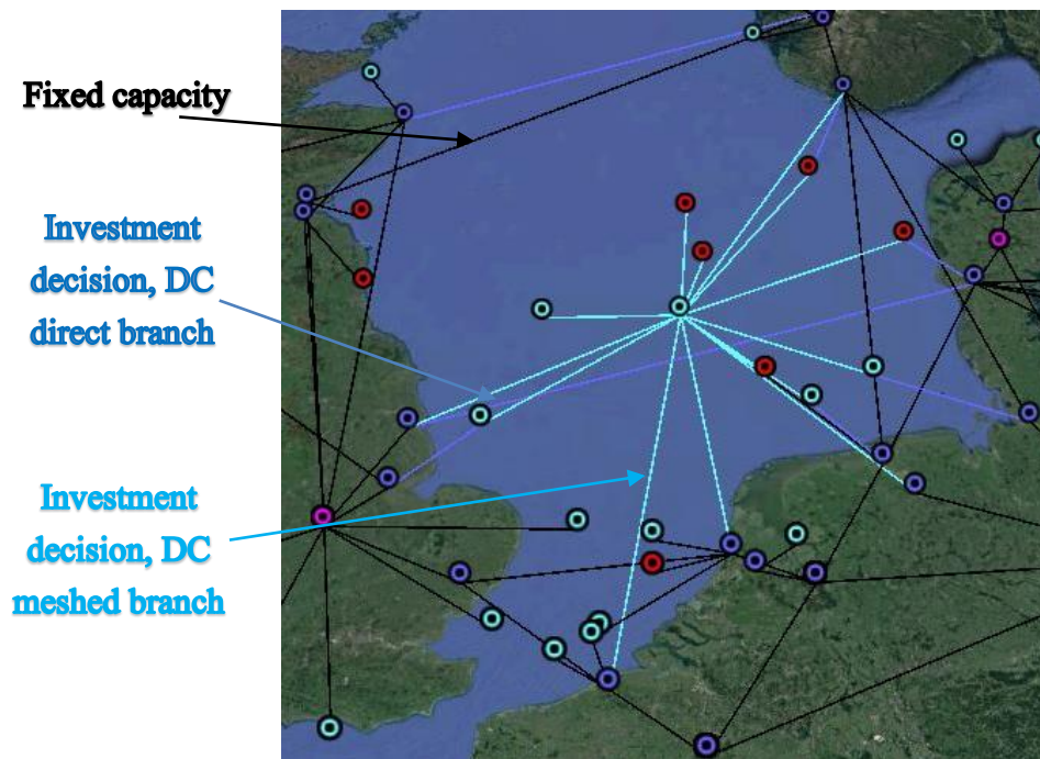
Figure 37. Obtained grid layout for scenario 4. (a, b, c, d and e analysis)
