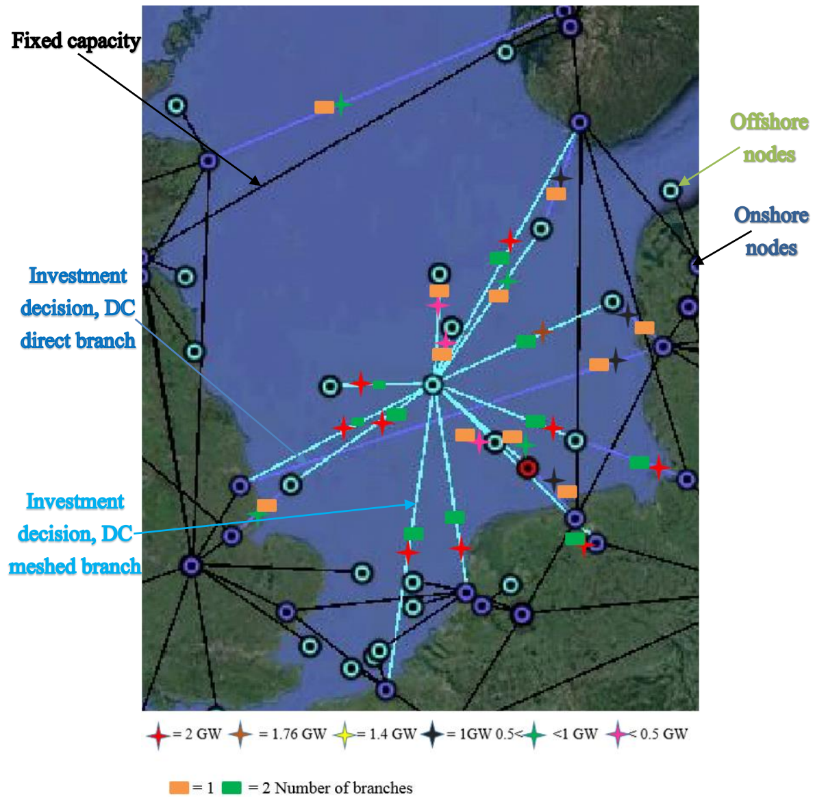
Figure 48. Chosen offshore grid layout for scenario 4.
