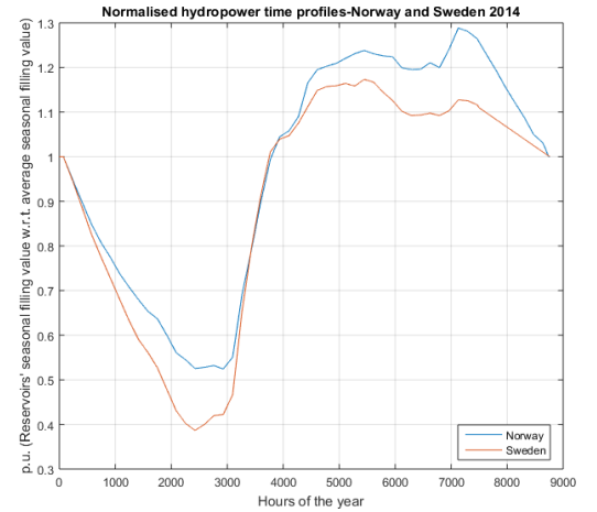
Fig. 4. Created Storage Time Profiles 2014
