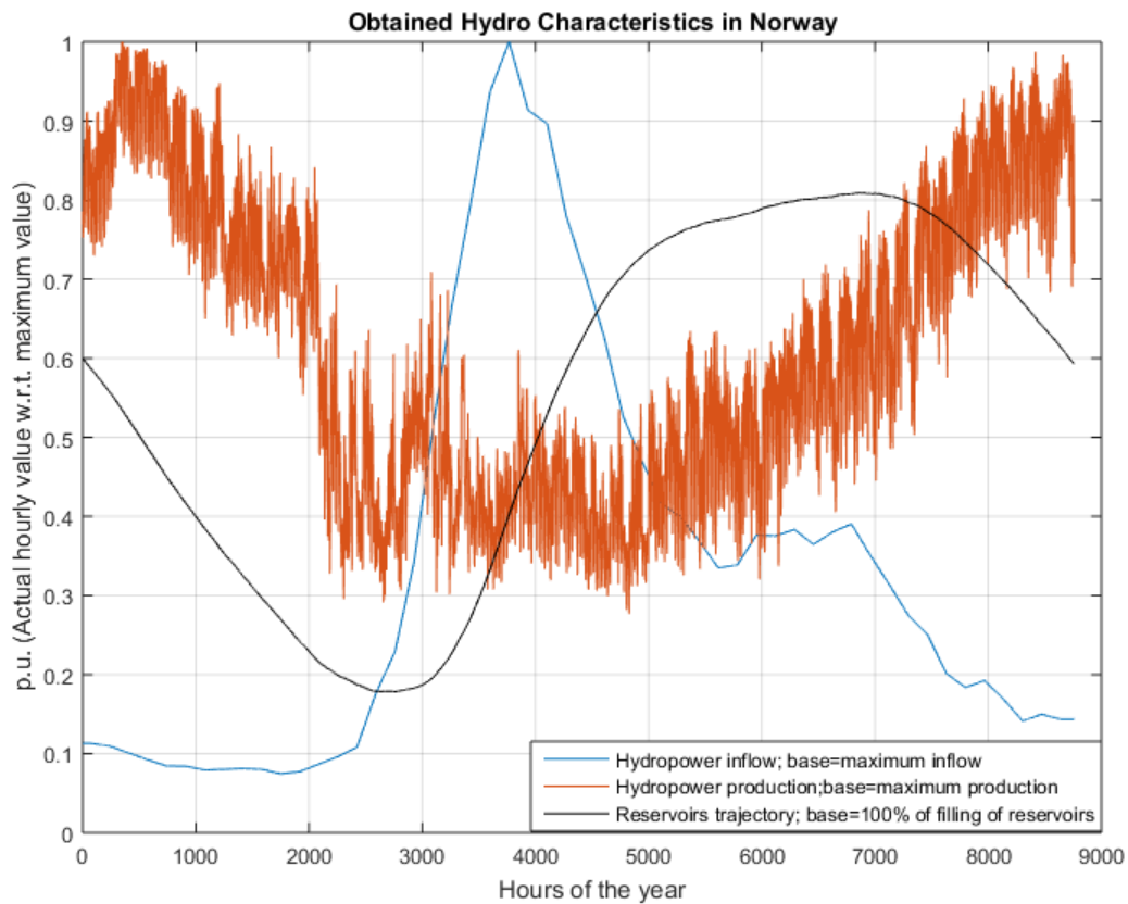
Figure 25. Obtained hydro characteristics in Norway.
