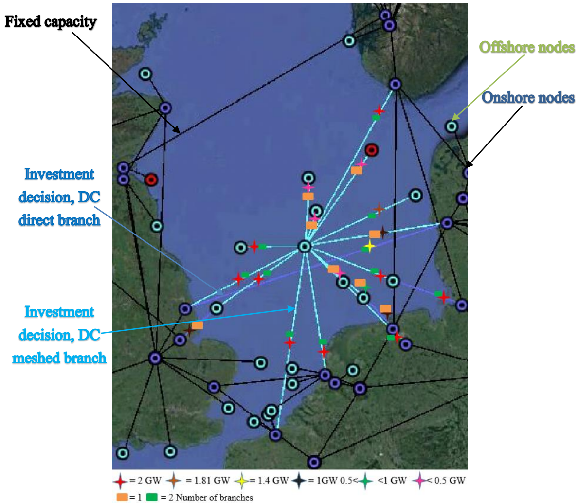
Figure 60. The most robust grid layout w.r.t. future energy scenarios.
