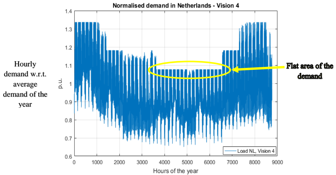
Figure 33. Actual normalised load profiles in Netherlands, scenario 4.
