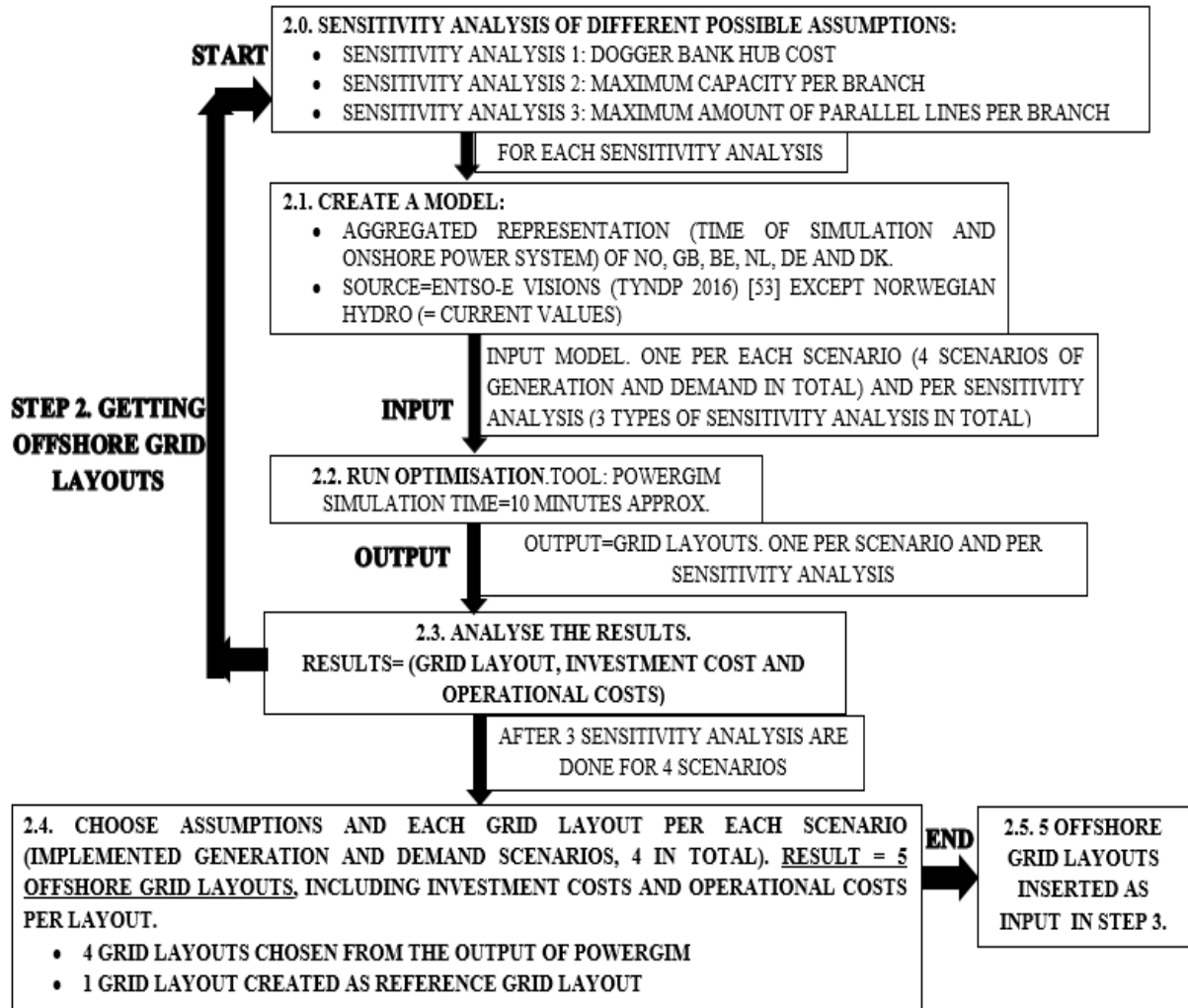
Figure 2. Flow chart of the second step of this Master Thesis.
