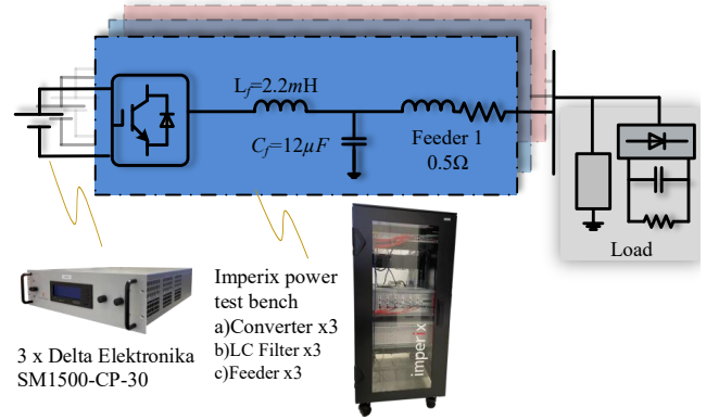
Fig. 6. Experiment setup.
