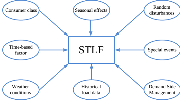
Fig. 1. Input parameters for training data [Note: Consumer class, random disturbances and demand side management are excluded in this study]
