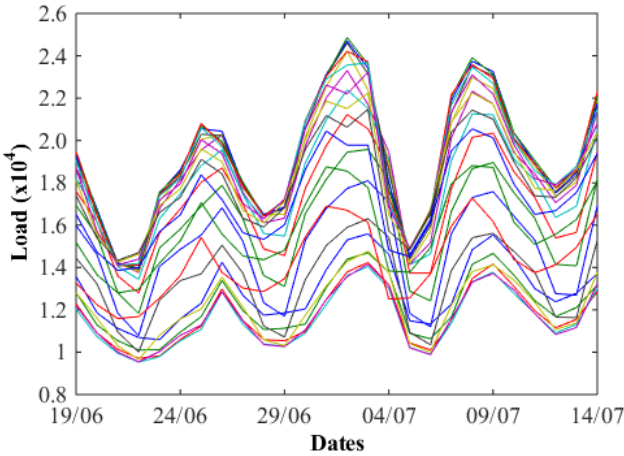
Fig. 5. Hourly load forecast for date range (19/06/2014 – 14/07/2014)
