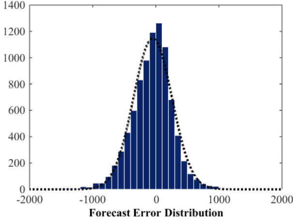
Fig. 9. Histogram and normal distribution fit of forecasted error with \mu = -61.89 and \sigma = 351.35
