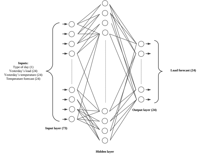
Fig. 2. Neural network architecture for short-term load forecast
