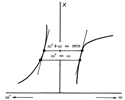
Fig. 28. \omega and \omega' as functions of x .
