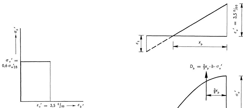
Fig. 30. Simplified stress-strain diagram for concrete.
