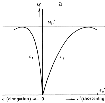
Fig. 5a. Diagrammatic representation of the relation between N' , \varepsilon_1 and \varepsilon_2 .
