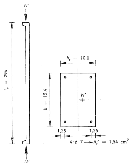
Fig. 16a. Columns tested by GAEDE (Report 129 D.A.f.S.) – dimensions in cm.
