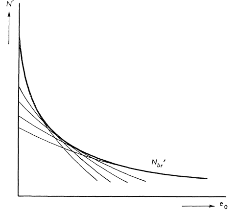
Fig. 6. Envelope formed by lines of constant value of \varepsilon_2 and indicating the relation between the ultimate load N_{br}' and the initial eccentricity e_0 for a member with given dimensions.
