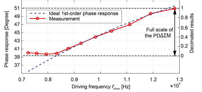
Fig. 12. Measured phase shift as a function of the drive frequency.
