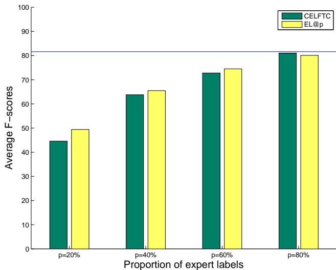
Fig. 7. Average f-scores ( f_{avg} ) for detecting a build for CELFTC: MSS and audio features at different proportions of expert labels. The horizontal blue line indicates the performance of the baseline event detector with 100% expert labels.
