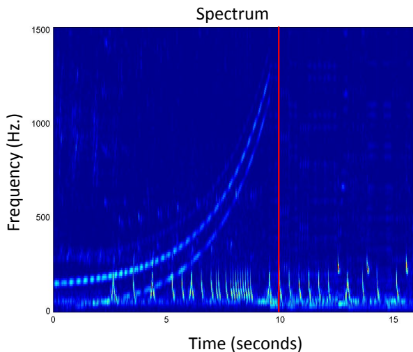
Fig. 5. Spectrogram of a segment containing a drop . One can observe a sweep-like structure on the left side of the figure. The red vertical line indicates the position of the drop.
