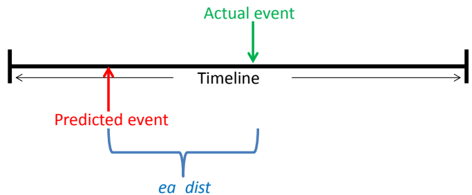
Fig. 2. Visualisation of the event anticipation distance ( ea\_dist ) metric useful to evaluate jump-in points provided to the listener in a non-linear access scenario.
