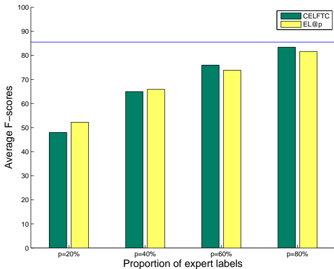
Fig. 6. Average f-scores ( f_{avg} ) for detecting a drop for CELFTC: FLS and image features at different proportions of expert labels. The horizontal blue line indicates the performance of the baseline event detector with 100% expert labels.
