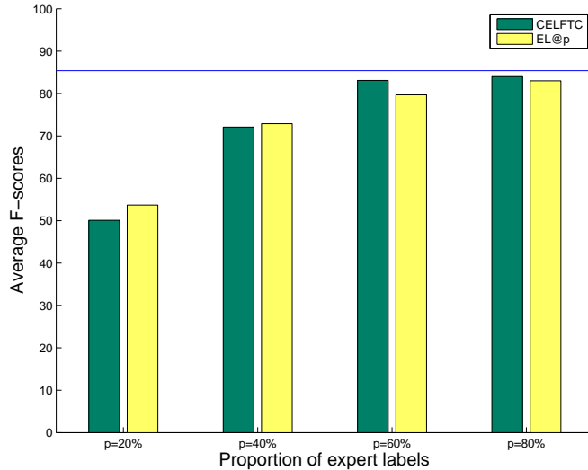
Fig. 8. Average f-scores ( f_{avg} ) for detecting a break for CELFTC: MSS and image features at different proportions of expert labels. The horizontal blue line indicates the performance of the baseline event detector with 100% expert labels.
