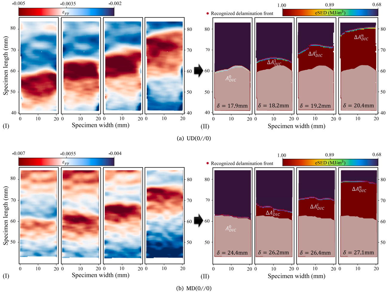
Fig. 2. Monitoring delamination growth by implementing DIC-eSED method for (a) UD(0/0) and (b) MD(0/0) specimens. (I) Longitudinal strain \epsilon_{yy} field at different delamination stages. (II) Calculated eSED field with recognized delamination front denoted by red dots. The area (dark red) below the delamination front is the fully delaminated region. Delamination growth of the i th measurement \Delta A^i_{DIC} = A^i_{DIC} - A^0_{DIC} ( i = 1, 2, \dots, n ). A^0_{DIC} is the initial delamination area after pre-cracking. (For interpretation of the references to colour in this figure legend, the reader is referred to the web version of this article.)
