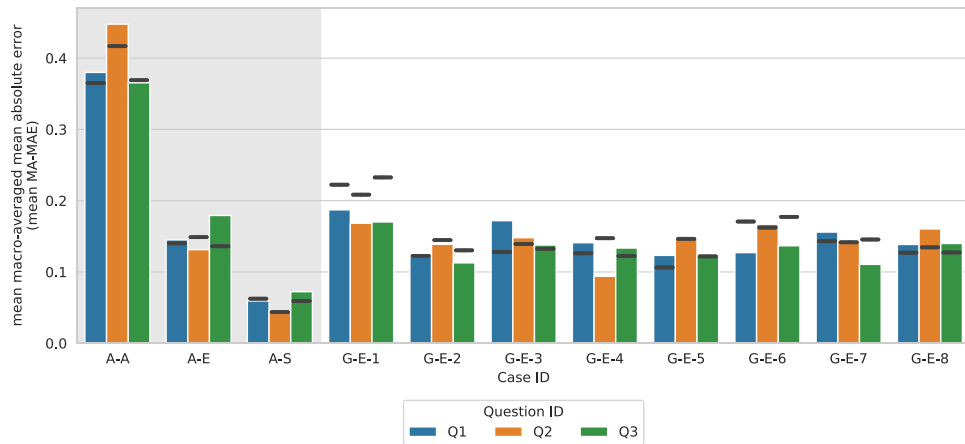
Figure 14. Mean macro-averaged MAE performance measures for testing data (bars) and fitting data (horizontal lines). White background highlights the generalizability (G) cases.
