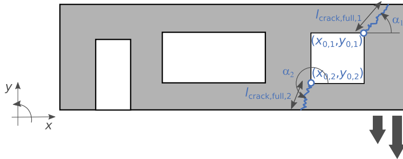
Figure 7. Crack parametrization for the facade of a typical Dutch masonry dwelling (facade ID: 1) under damage cause 2 (pattern ID: 102).
