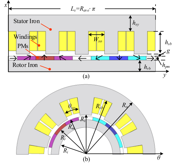
Fig. 2. Analytical model for AFPM machine. (a) Analytical model in Cartesian coordinates. (b) Converted model in polar coordinates.
