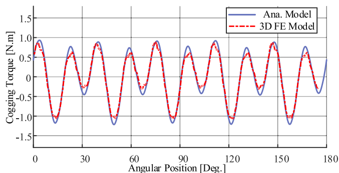
Fig. 16. Comparison of cogging torque under partial demagnetization.
