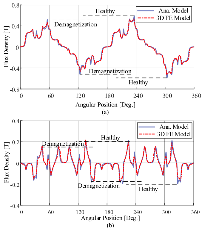
Fig. 13. Total airgap flux density waveforms under partial demagnetization. (a) Radial component. (b) Tangential component.
