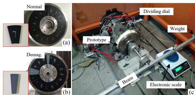
Fig. 17. Prototype machine and the experimental set-up. (a) Normal. (b) Demagnetization. (c) Cogging torque test.
