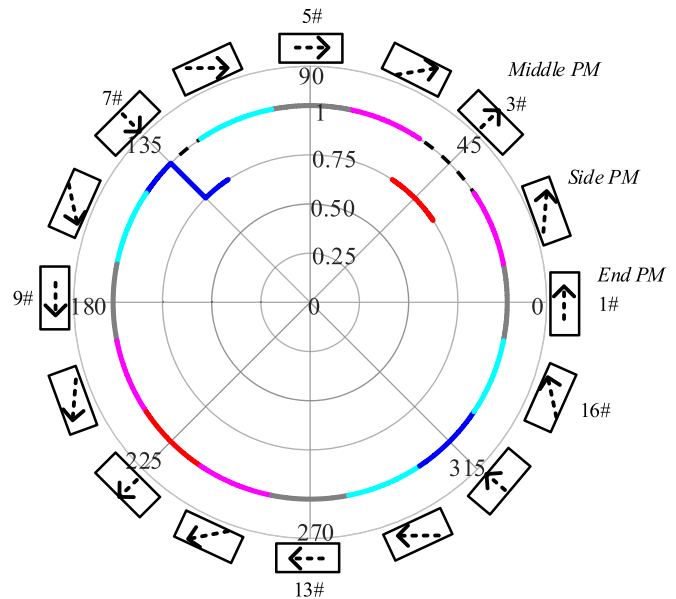
Fig. 11. Space distribution of PM remanence.
