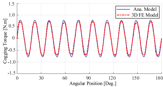
Fig. 10. Comparison of cogging torque.
