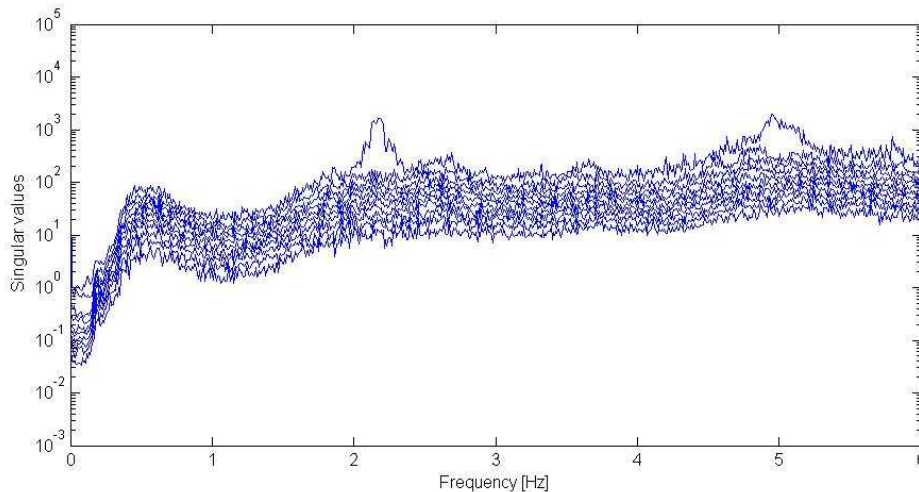
Fig. 9 – Singular value spectrum of the PSD's of all sensor data combined
