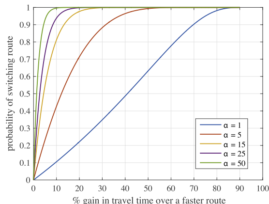
Fig. 4. Influence of route selection parameter on switching probability to a faster route.
