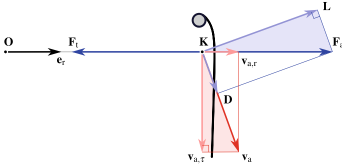
Fig. 7.12 Quasi-steady force equilibrium governing the flight motion of a massless kite, with apparent wind velocity components \mathbf{v}_{a,\tau} and \mathbf{v}_{a,r} , and aerodynamic force components \mathbf{L} and \mathbf{D} , in the plane spanned by the apparent wind velocity \mathbf{v}_a and the resultant aerodynamic force \mathbf{F}_a
