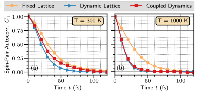
FIG. 4. Spin pair autocorrelation functions of CrN at T = 300 K (a) and T = 1000 K (b) obtained from ASD (fixed lattice), ASD on a pre-calculated DLM-AIMD vibrating lattice (dynamic lattice) and ASD-AIMD (coupled dynamics).
