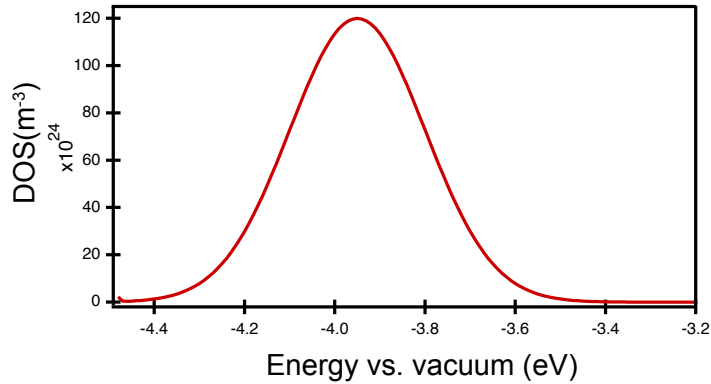
Figure A4.3 Density of states function used in the simulations. Levels more than ~1 eV above the bandgap are not considered as they will not be relevant for the applied potentials simulated here.
