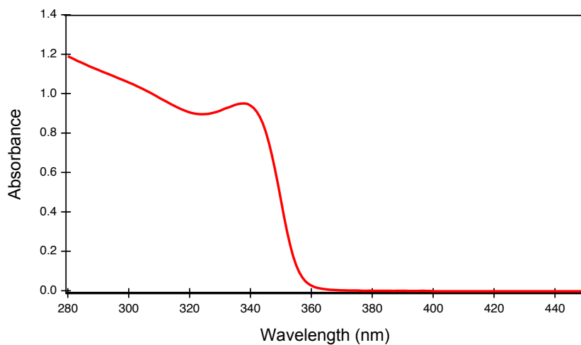
Figure A4.1 The absorption spectrum of ZnO QDs dispersed in ethanol.
