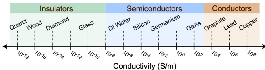
Figure 1.1 Room temperature conductivity of typical insulator, semiconductor, and conductor materials. DI water stands for deionized water.
