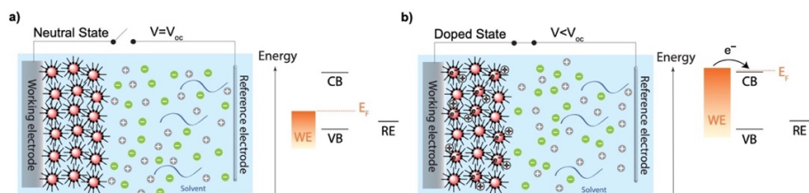
Figure 2.1. Schematic of electrochemical charge injection into QD film. (a) shows a situation where the Fermi level is inside the band gap of the QD when there is no applied potential to the WE, (b) shows a situation where the Fermi level in this case is above the conduction band of the QD as a function of applied negative potential with respect to RE. To neutralize the injected electrons electrostatically, electrolyte cations diffuse into the voids of QD film.
