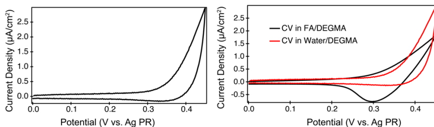
Figure A3.2 CV of P3DT film scanned outside of the glove box in an electrochemical cell containing 0.05 M AMPSH dissolved in water/DEGMA mixture (left), comparison of CVs taken inside (FA/DEGMA) and outside (water/DEGMA) of glove box for P3DT film (right).
