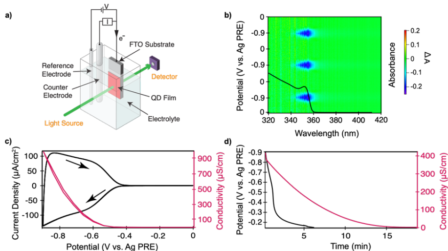
Figure 2.2. (a) The schematic of spectro-electrochemistry cell set-up with three-electrode configuration for in-situ optical absorbance measurement, (b) the 2D color map showing the differential absorbance, bleach ( \Delta A ) from ZnO QD film during electrochemical charging and discharging (with a scan rate of 50 mV/s), with an absorption spectrum (black line) of the film on top of it, (c) the CV of the ZnO QD film scanned starting around 0 V to -0.9 V vs Ag PRE with a scan rate of 50 mV/s (black line) and the conductivity of the same film as a function of applied potential (red line), (d) both conductivity (red line) and Fermi-level stability (black line) measurements over time after disconnecting the cell from the potentiostat. All measurements are performed in an electrolyte solution containing 0.1 M LiClO 4 in ACN.
