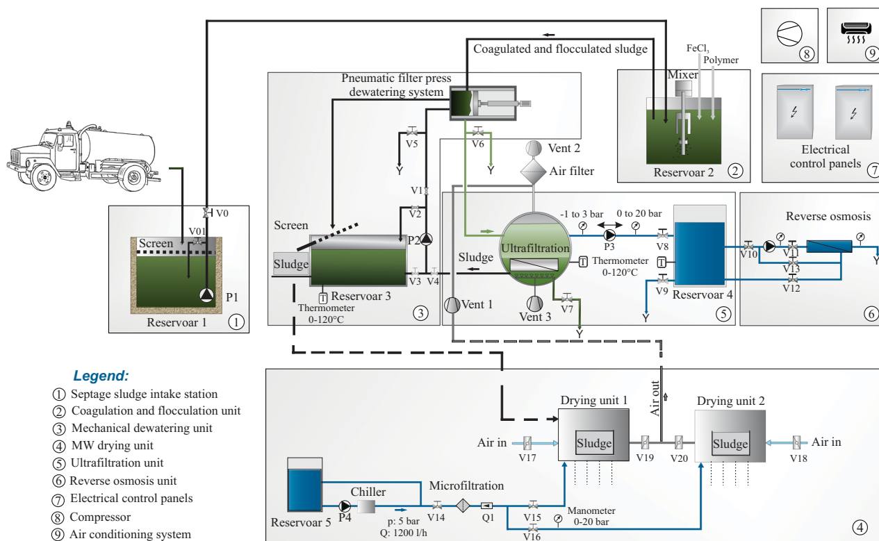
Technological scheme
