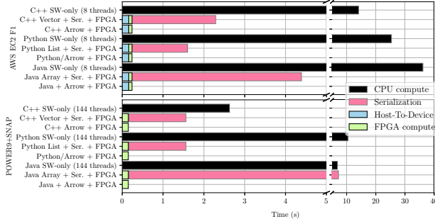
Fig. 5. Run-time components of regular expression matching accelerator
