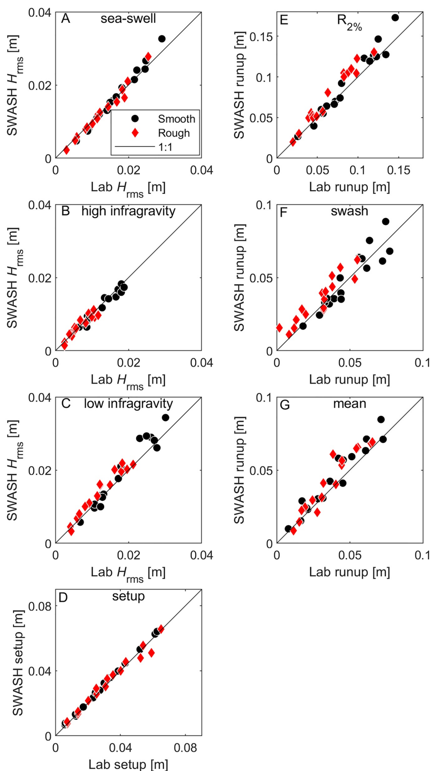
Figure 5. Comparison between observed and predicted (a) sea-swell, (b) high infragravity, and (c) low infragravity rms wave heights, and (d) wave setup at the directional wave gauge nearest the shoreline ( x = 10.75 m). Comparison between observed and predicted (e) 2% exceedance runup and its components (f) 2% exceedance swash and (g) the mean components (wave setup at the shoreline). All smooth (black circles) and rough (red diamonds) runs (Table 1) are shown.
