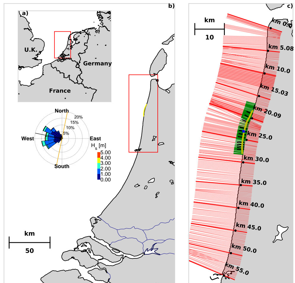
Figure 2. Location of case study site and an overview of the survey transects from available datasets. (a) Location of Dutch coastline within Europe. (b) Location of Hondsbosse Dunes nourishment (yellow line) at the Dutch coast including local nearshore wave climate at HD at -10\text{ m} + \text{NAP} depth based on a 20-year hindcast time-series derived by Kroon et al. [36]. (c) Location of transects from Jarkus (red), contractor survey transects (green), and 11 constructor high-temporal-resolution transects (black); the blue star indicates the location of the nearshore wave climate.
