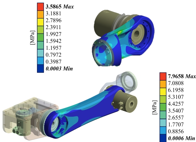
Figure 7: FE analysis and topology optimization results.
