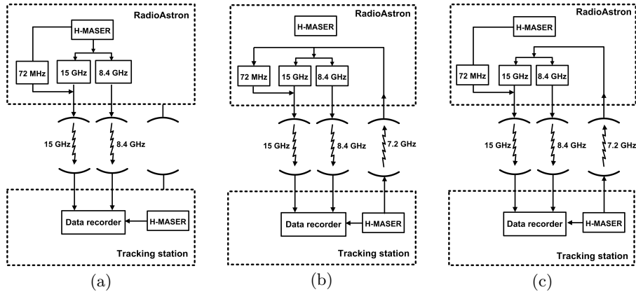
Figure 1: On-board hardware synchronization modes. (a) “H-Maser”. (b) “Coherent”. (c) “Semi-Coherent”. Note that, due to a fixed architecture of the RadioAstron on-board radio system, the 8.4 GHz tone and the carrier of the 15 GHz data link must use one and the same reference signal at any given time: either from the on-board H-maser or from the tracking station uplink.
