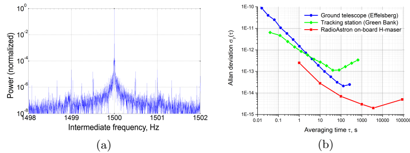
Figure 2: Frequency stability of the 8.4 GHz RadioAstron downlink signal. (a) Phase-stopped signal spectrum (data recorded by the Effelsberg telescope, 2015/11/19). (b) Comparison of the frequency stability in terms of the Allan deviation of the signal recorded by a radio telescope (blue, circles) and a tracking station (green, diamonds). Allan deviation of the on-board H-maser obtained during laboratory tests (red, squares).
