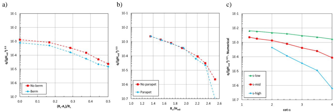
Figure 1. Numerical non-dimensional overtopping discharges as function of a) the protruding part of the crest wall (R_c - A_c)/R_c , b) the addition of a recurved parapet, and c) the slope angle \cot \alpha
