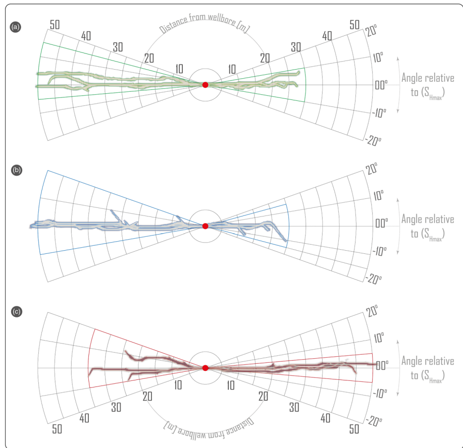
Figure 11. A comparison of hydraulic fracture simulation V-pf models for (a) the limestones (green color); (b) the marbles (blue color); (c) the skarns (red color); hydraulic fracture lengths are given by the concentric dividers, and hydraulic fracture angles compared to S_{Hmax} 's orientation is given by the radial dividers.
