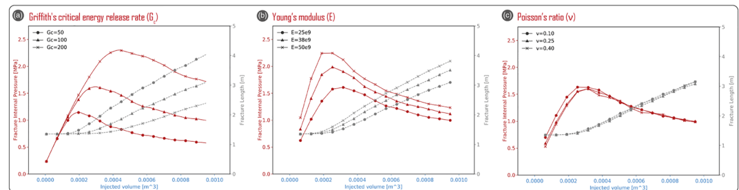
Figure 4. Sensitivity analysis of mechanical material properties. The plots report the evolution of fracture internal overpressure (reds) and fracture length (grays) against the injected volume: in (a) for different values of the critical energy release rate of the bulk solid G_c = 50, 100, 200 \text{ Pa m}^{-1} ; in (b) for different elastic parameters of Young's modulus with E = 25, 38, 50 \text{ GPa} ; and (c) different Poisson's ratio \nu = 0.10, 0.25, 0.40 .
