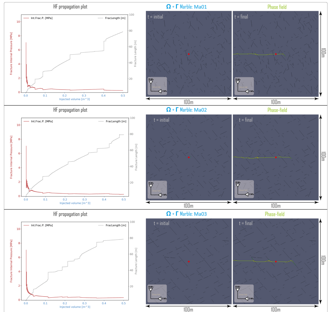
Figure 9. Hydraulic fracture models using V-pf with the sub-DFN of the marble reservoir. The matrix material domain \Omega is represented in gray; the natural fractures \Gamma are discretized in black. Ma01 is composed with 295 natural fractures, Ma02 is composed with 215 natural fractures, and Ma03 is composed with 198 natural fractures. The stress field is oriented such that S_{Hmax} is aligned along the horizontal direction. The red dots represent the well-bore and initial fracture position (and initial phase-field implementation).
