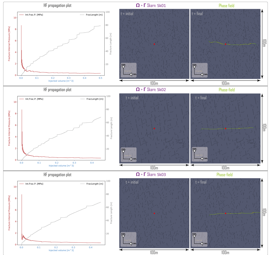
Figure 10. Hydraulic fracture models using V-pf with the sub-DFN of the skarn reservoir. The matrix material domain \Omega is represented in gray; the natural fractures \Gamma are discretized in black. Sk01 is composed with 706 natural fractures, Sk02 is composed with 495 natural fractures, and Sk03 is composed with 375 natural fractures. The stress field is oriented such that S_{Hmax} is aligned along the horizontal direction. The red dots represent the well-bore and initial fracture position (and initial phase-field implementation).
