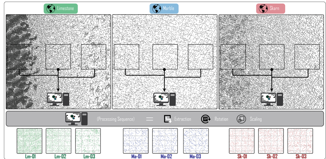
Figure 3. This figure presents the preprocessing sequence: from original reservoir scale DFN, to extracted, rotated, and scaled models to fit the numerical analyses requirements. From left to right, the DFN for the Limestone formation, the DFN for the marble formation and the DFN for the skarn formation. Symbols Lm/Ma/Sk-01, Lm/Ma/Sk-02, and Lm/Ma/Sk-03 are referred to the sub-DFN extracted from initial DFN.
