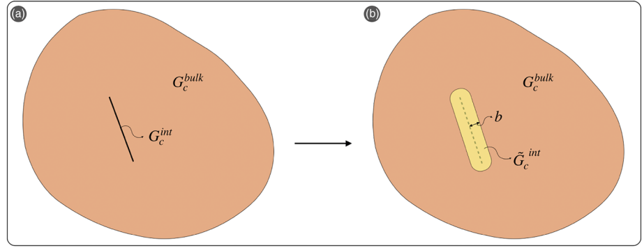
Figure 2. (a and b) Diffused representation of a discontinuous interface.
