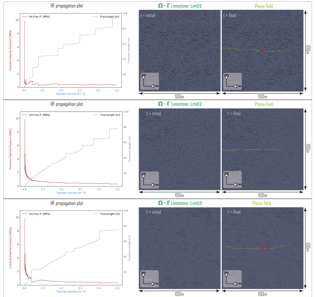
Figure 8. Hydraulic fracture models using V-pf with the sub-DFN of the limestone reservoir. The matrix material domain \Omega is represented in gray, the natural fracture \Gamma are discretized in black. Lm01 is composed with 1,483 natural fractures, Lm02 is composed with 709 natural fractures, and Lm03 is composed with 327 natural fractures. The stress field is oriented such that S_{Hmax} is aligned along the horizontal direction. The red dots represent the well-bore and initial fracture position (and initial phase-field implementation).
