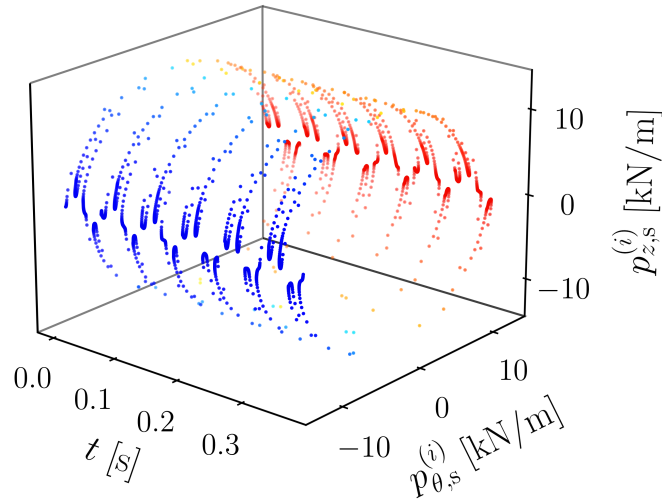
Figure 7: Friction force trajectory at z_i = 3.0 m and u_R = 5.5 m; the color of the markers is based on the ratio of circumferential to total friction force, i.e. ranging from -1 (blue) to 1 (red).
