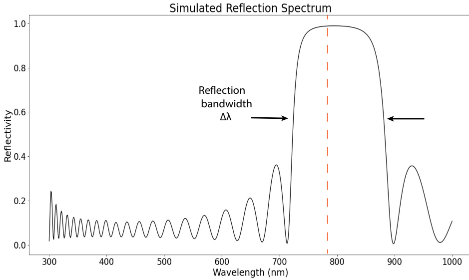
Figure 5.4: Simulated spectrum of 21 layers of \text{SiO}_2 and \text{Si}_3\text{N}_4 forming a quarter wave stack for light around 795 nm. Reflectivity at 795 nm (indicated by the dashed line) is above 99%. The reflection spectrum is created using the OpenFilters Software package for thin film design [40].
