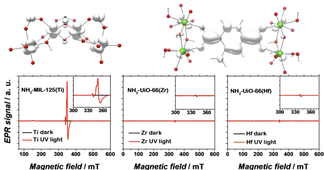
Figure 3. EPR spectra of dark ( black ) and UV-illuminated ( red ) MOFs: \text{NH}_2\text{-MIL-125(Ti)} ( left ), ‘ideal’ \text{NH}_2\text{-UiO-66(Zr)} ( centre ) and \text{NH}_2\text{-UiO-66(Hf)} ( right ). The photoexcited electron is primarily Ti-centred in the case of \text{NH}_2\text{-MIL-125} , whereas in the UiO-type materials, the electron resides on the organic linker.
