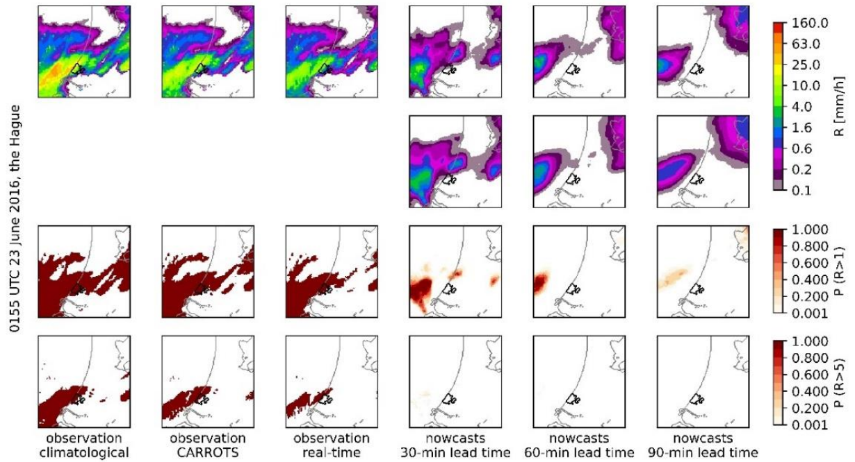
FIG. 5. Climatological, CARROTS-adjusted, and real-time radar QPE and nowcasts with 30-, 60-, and 90-min lead time for the rainfall event in the Hague from 0155 UTC 23 June 2016 to 0255 UTC 2016. Upper 2 rows: rainfall intensity. The shown rainfall intensity is the average intensity during the 1-h event.
