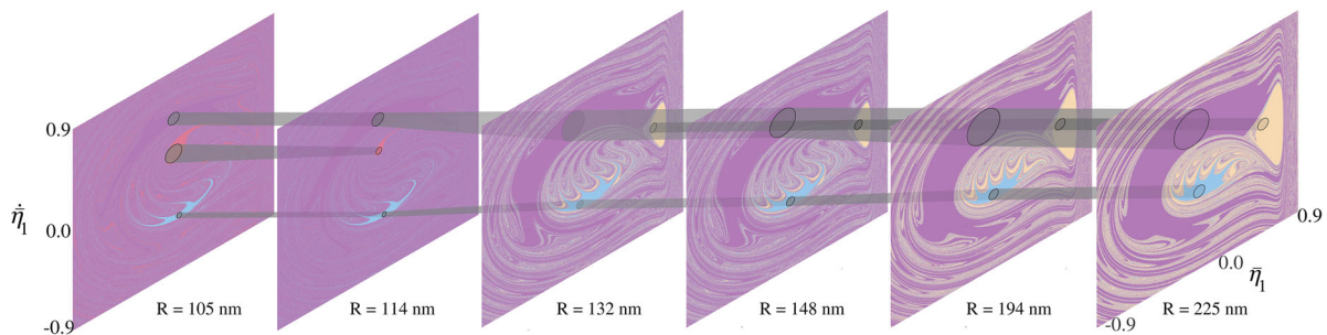
Fig. 9 Phase-space topology evolution with respect to tip radius ( R ) from 105 to 225 nm, at fixed excitation amplitude and frequency of \bar{y} = 0.020 , \bar{\Omega} = 0.8 , respectively
