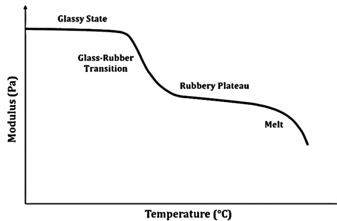
Figure 1.9. Schematic illustration of modulus-temperature relationship of semi-crystalline thermoplastics (adapted from [3]).
