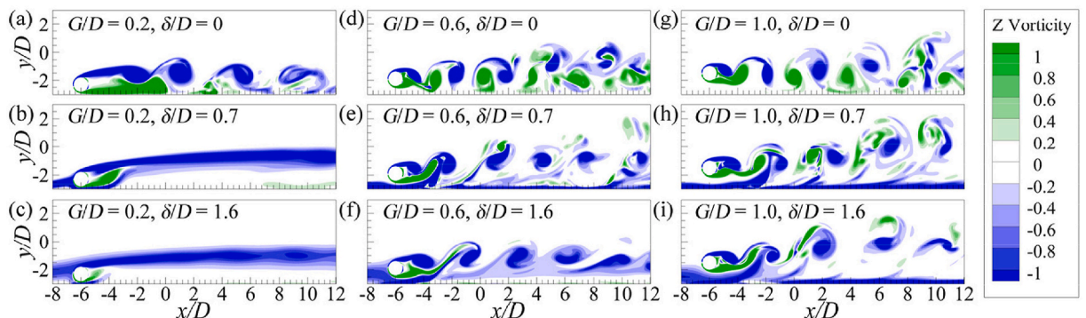
Fig. 13. Time history of non-dimensional spanwise vorticity contours for various G/D and \delta/D for Re = 350 (Zhang et al., 2021).
