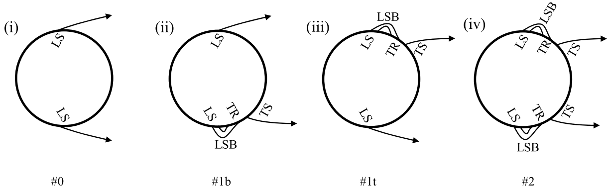
Fig. 12. Representation of flow behind the cylinder displaying (i) no bubble (ii) bubble on the bottom (iii) bubble on top (iv) bubble on both sides of the cylinder. LS, TS, and TR represent Laminar separation, Turbulent Separation, and Turbulent Reattachment, respectively (Desai et al., 2020).
