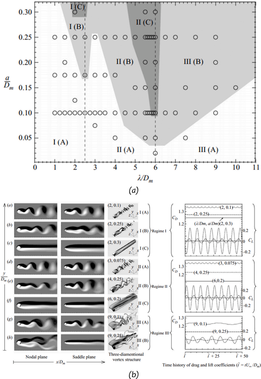
Fig. 26. Flow patterns (a) Flow pattern regimes (b) Flow patterns for SW cylinders for different a/D_m and \lambda/D_m at Re = 100 (Note: Symbol (○) in (a) presents each SW cylinder) ( Lam and Lin, 2009 ).
