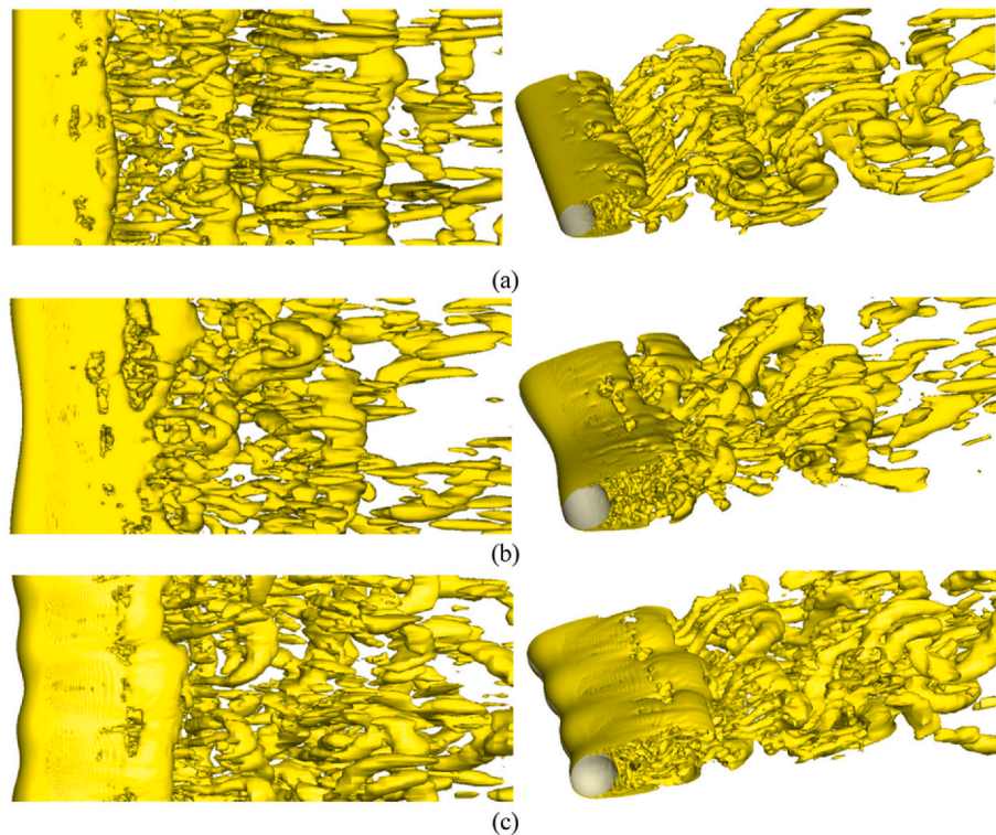
Fig. 29. Left: top view and right: perspective view of the iso-surface vortex shedding around (a) circular cylinder, (b) SW cylinder, and (c) DW cylinder at Re = 3.0 \times 10^3 (Yoon et al., 2020).
