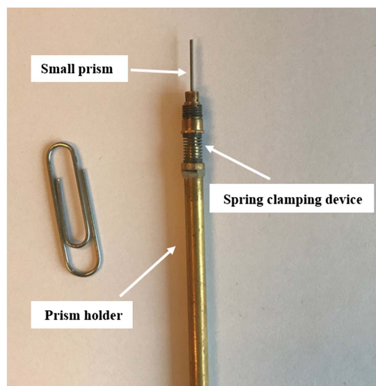
Fig. 1. Microbeam specimen clamped on the holder prior to X-ray computed tomography experiment. (Reprinted from Cement and Concrete Research , Vol. 102, H. Zhang, B. Šavija, S. Chaves Figueiredo, and E. Schlangen, “Experimentally validated multi-scale modelling scheme of deformation and fracture of cement paste,” pp. 175–186, © 2017, with permission from Elsevier.)
