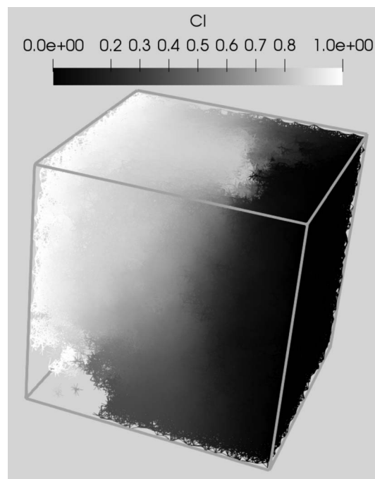
Fig. 15. Chloride distribution in cement paste under an imposed concentration gradient in the Z-direction.
