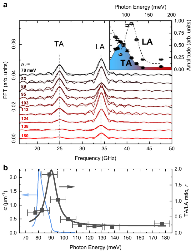
Fig. 4 Tunable shear strain. a Fourier transforms of the measured polarization rotation signals corresponding to strain wave propagation after excitation with different pump energies h\nu . Inset: Pump photon energy dependent amplitude of the two oscillations corresponding to LA and TA strain waves for fixed pump and probe polarizations as obtained from the Fourier transforms shown in panel a . The solid and dashed lines are guides to the eyes. The errorbars account for the uncertainty of the fit. b Linear absorption due to the infrared-active phonon modes, as taken from ref. 14 (left axis) and ratio r of the TA and LA mode amplitudes (right axis) vs photon energy at constant incident fluence. The black line serves as a guide to the eye. The spectral full-width at half-maximum of the excitation pulses is indicated by the errorbars.
