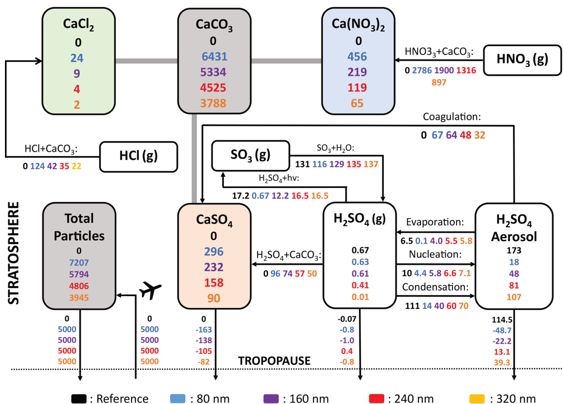
Figure 9. The stratospheric sulfur cycle under conditions of SAI of 5 Mt yr -1 calcite particles with radii of 80 (blue), 160 (violet), 240 (red) and 320 nm (orange). All sulfur species (except CaSO 4 ) are shown in Gg S for burden (boxes) and Gg S yr -1 for net fluxes (arrows). The solid species (coloured boxes) are given in Gg of the corresponding material. The HNO 3 and HCl flux to Ca(NO 3 ) 2 and CaCl 2 are given in Gg HNO 3 yr -1 and Gg HCl yr -1 . Cross-tropopause fluxes are calculated by balancing the mass balance of the individual species.
