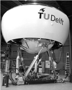
Fig. 3. The SIMONA Research Simulator.
