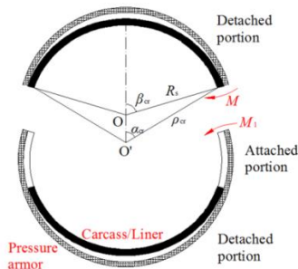
FIGURE 9: BENDING MOMENTS AT THE CONTACT POSITION
