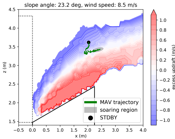
Fig. 8. Flight trajectory during the autonomous search, from 352 to 537 seconds in case I. The MAV started searching at the standby position (STDBY), marked as a black dot. It found a good soaring location and achieved zero throttle in 185 seconds.
