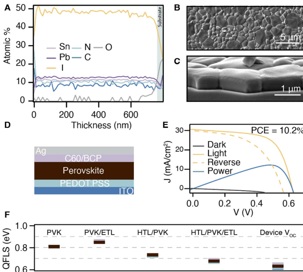
Fig. 1 (A) Compositional XPS depth profiles showing the atomic percentage (%) as a function of the layer thickness (nm) of FAPb 0.5 Sn 0.5 I 3 PVK films deposited in a single cycle of sequential thermal evaporation. (B) Top-view SEM image of an annealed PVK film. The scale bar indicates 5 μm. (C) Cross-sectional SEM images of an annealed PVK film. The scale bar indicates 1 μm. All samples used were annealed for 30 minutes at 200 °C. (D) Schematic representation of the device architecture used in this work, consisting of ITO/PEDOT:PSS/FAPb 0.5 Sn 0.5 I 3 /C60/BCP/Ag. (E) J–V and power characteristic of the champion cell employing 500 nm thick PVK films. The reverse scan is also included. (F) Quasi-Fermi level splitting (QFLS) of the bare PVK film as well as the partial stacks with the HTL (PEDOT:PSS) and the ETL (C60). Plotted together with the device open-circuit voltage ( V_{OC} ).
