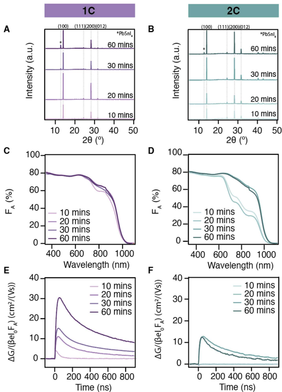
Fig. 2 XRD patterns of FAPb 0.5 Sn 0.5 I 3 perovskite films deposited in (A) a single cycle (1c) and (B) a double cycle (2c) of sequential thermal evaporation. Absorption spectra, expressed as the fraction of absorbed light ( F_A , %) of the (C) 1c deposition and (D) 2c deposition. Time-resolved photoconductance measurements of the (E) 1c deposition and (F) 2c deposition. The photoconductance ( \Delta G ) is normalized by a geometric factor ( \beta ), the elementary charge constant ( e ), the intensity of the incoming light pulse, and F_A . All measurements were carried out on samples that were annealed for 10, 20, 30, and 60 minutes, and using light intensities of 10^{10} photons per cm 2 .
