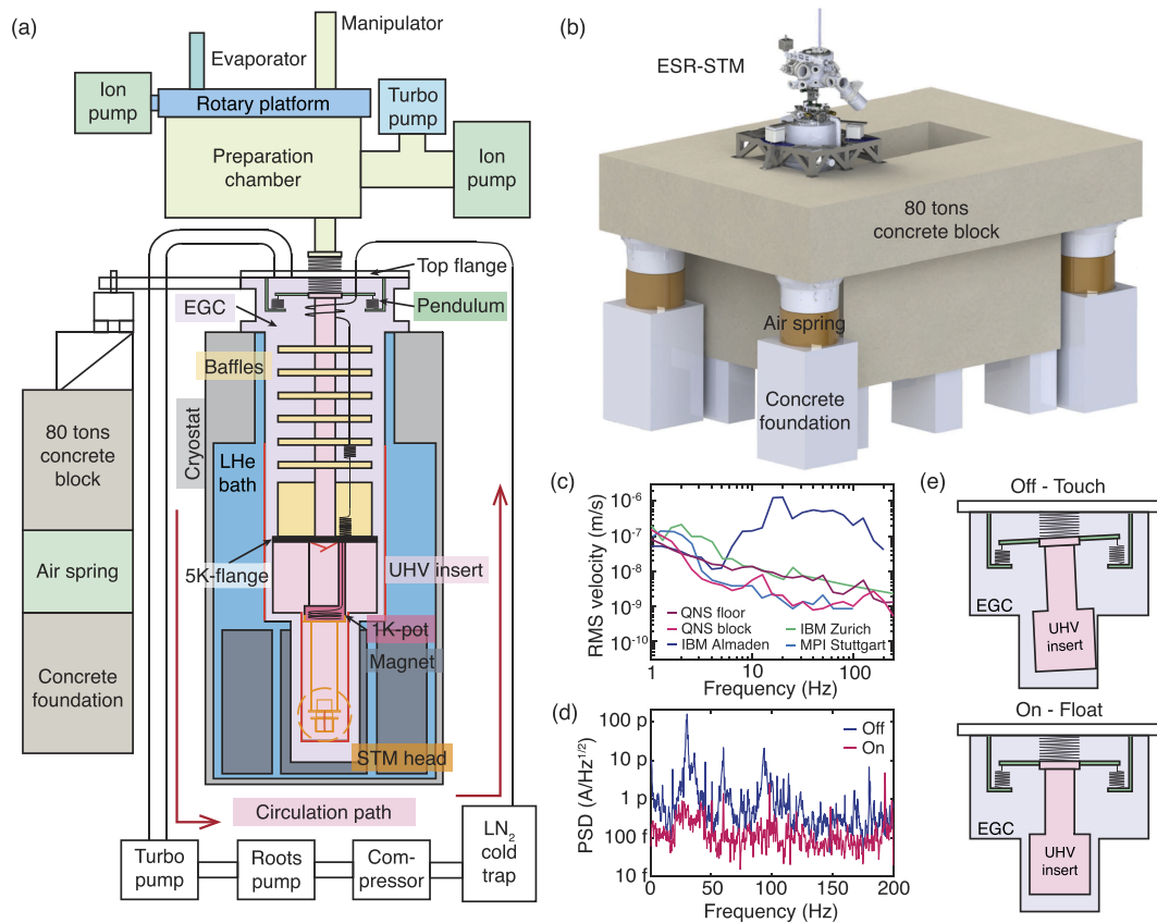
FIG. 1. Design of the homebuilt ESR-STM. (a) Overview of the whole system including a cryostat, a vector magnet, a mechanical damping system, a cooling system, an STM, and a preparation chamber. The preparation chamber and the ultrahigh vacuum (UHV) insert are connected to the top flange of an exchange gas can (EGC) via a flexible bellows. The UHV insert is supported by three arms connected to the system via three flexible bellows (labeled “Pendulum”). (b) ESR-STM setup on a massive concrete block. The cryostat rests on a concrete block floated by four air springs in a soundproof room. (c) Velocity spectrum measured on the floor of the soundproof room (purple, QNS floor) and on top of the floating concrete block (magenta, QNS block) in comparison with other precision laboratories (blue, IBM Almaden; green, IBM Zurich; light blue, MPI Stuttgart). (d) Power spectral density (PSD) of the tunnel current measured with pendulum on (magenta) and off (blue) ( V_{DC} = 10 mV, I = 1 nA, Integral-gain = 1 nm/s). (e) Schematics showing pendulum operation. The UHV insert is suspended by three welded bellows, while schematic shows only two bellows for simplicity. When the pendulum is in the “off” state (top), the UHV insert is misaligned and thus in mechanical contact with EGC. In the “on” state (bottom), the pendulum is aligned inside the EGC without touching the EGC and, thus, mechanically isolated from the rest of the system.
