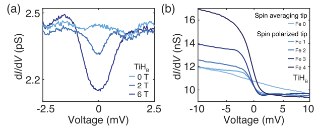
FIG. 7. Characterization of the TiH and the spin-polarized tip for ESR measurement. (a) dI/dV spectra of TiH B at different magnetic fields ( B_{\text{ext}} = 0, 2 , and 6 T) in the in-plane direction, V_{\text{DC}} = 4 mV, I = 70 pA, V_{\text{mod}} = 50 \mu V, T = 1.3 K). (b) dI/dV spectra of TiH B with different spin polarization of the tip. The spin-averaging tip corresponds to the Ag-coated STM tip. The STM tip is spin-polarized by picking up Fe atoms on the surface. Each spectrum was measured after picking up Fe atom one-by-one [five spectra measured with zero (spin-averaging tip, light blue) to four Fe atoms (spin-polarized tip, dark blue) at the tip apex] ( B_{\text{ext}} = 0.9 T, in-plane direction, V_{\text{DC}} = 10 mV, I = 100 pA, V_{\text{mod}} = 1 mV, T = 1.3 K).
