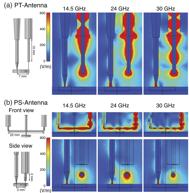
FIG. 4. COMSOL simulations of electric field distribution. (a) Schematics of the simulation setup and the simulated images of electric fields around the antenna, tip, and sample for the PT- and (b) PS-antenna when oscillating voltage signals are applied through the antennas. Three selected simulation results are shown when the frequency of the incident oscillating voltage is set to 14.5, 24, and 30 GHz.
