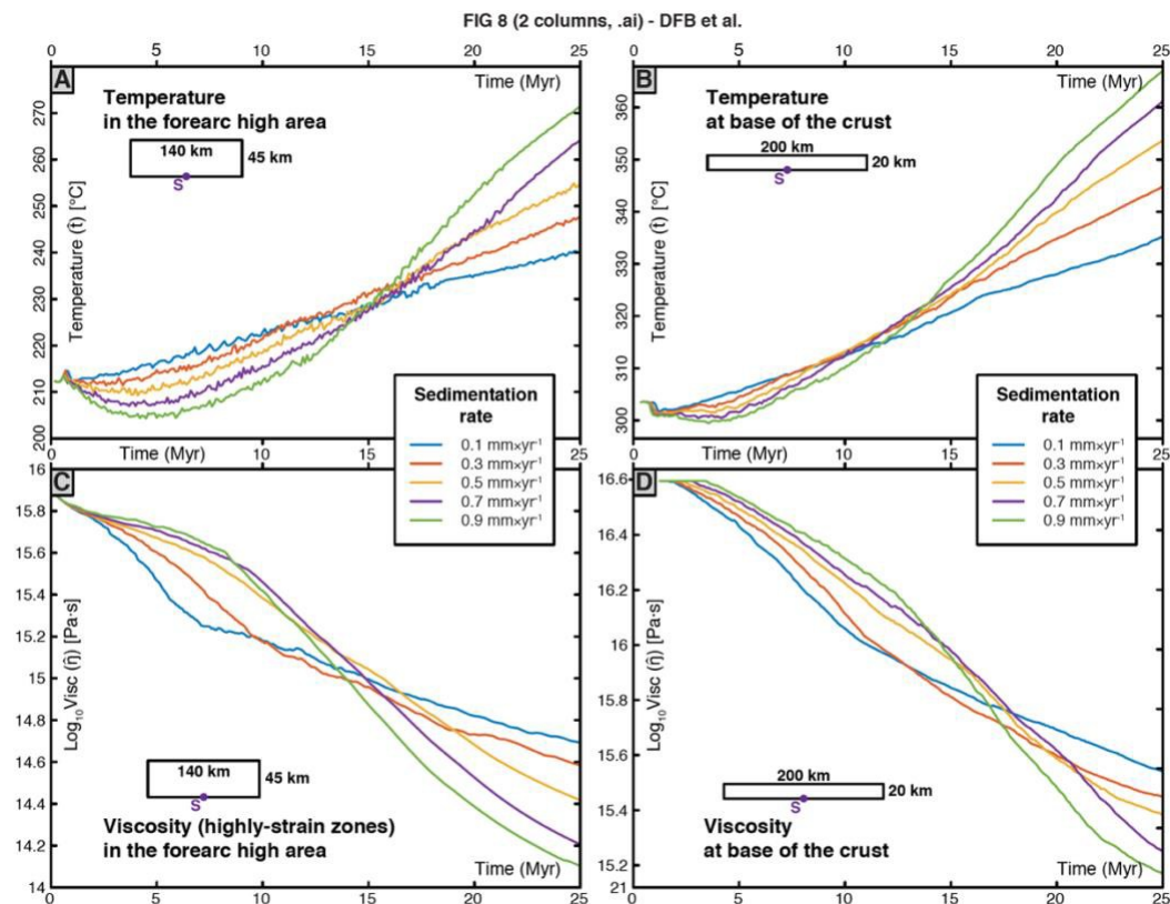
Figure 8. Temperature and viscosity variation of the forearc high and crustal base with sediment fill level. Evolution of median ( \bar{T} ) temperature and median ( \bar{\eta} ) viscosity in the forearc high region (A; C) and base of the crust (B; D). Areas considered are centred in the S point; 140 km wide x 45 km tall for the forearc high region and 200 km wide x 20 km tall for the base of the crust. We assure a representative, non-parametric calculus, using the median for both temperature field and viscosity distribution. For the former, we compute median temperature values for each grid point,
