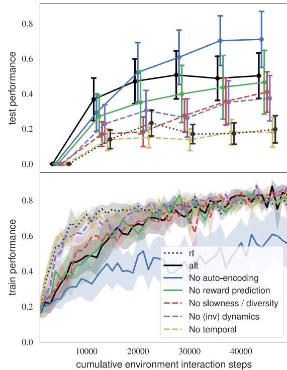
Fig. 5. The effect on the performance of the alt algorithm of turning off individual SRL losses. The no temporal experiment excludes both the (inv) dynamics and the slowness/diversity losses. The performance with all SRL losses ( alt ) and with no SRL losses ( rl ) are shown for comparison. The mean \pm half a standard deviation of the performance criterion from Section IV are shown.
