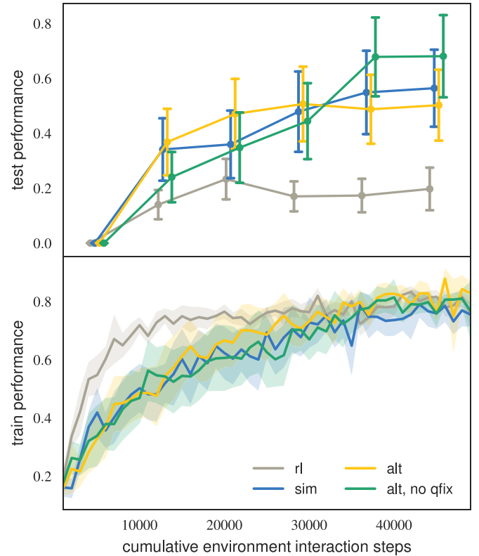
Fig. 3. Normalized performance for the rl , sim and alt methods, as well as the alt method without the \mathcal{L}_{\text{Qfix}} (11) loss term. For the test performance, every 10^4 steps the network parameters that gave the best training performance up to that point are evaluated on the test tracks, without any additional training on those tracks. The mean \pm half a standard deviation of the performance criterion from Section IV are shown.
