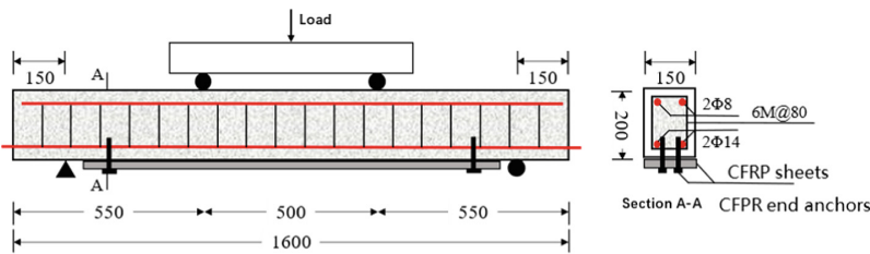
Fig. 1. Dimensions and reinforcement details of RC beams.
