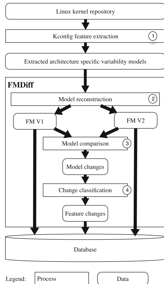
Fig. 2 Change extraction process overview
